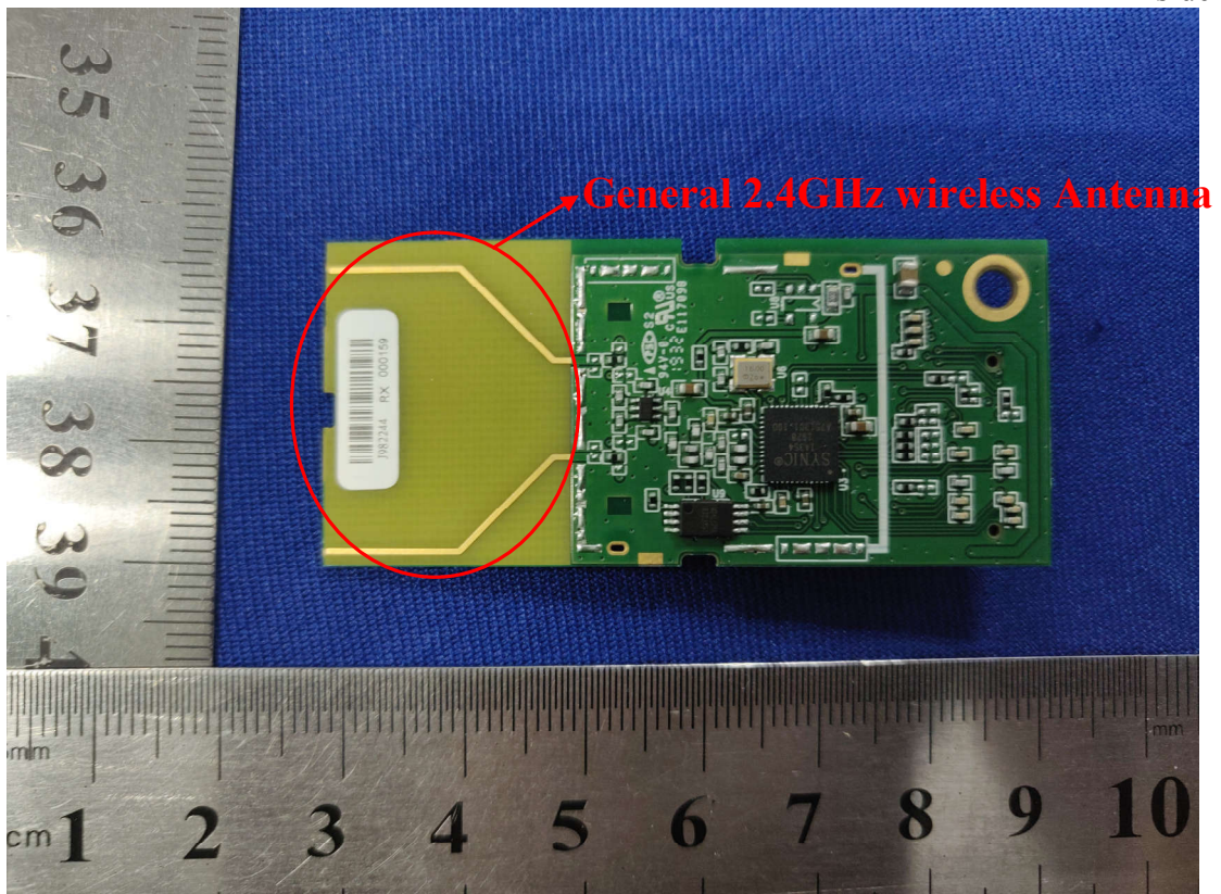
Figure 12 Inside of the EUT
