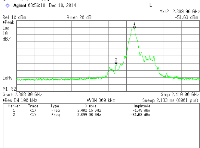
[BDR (DH3)]
