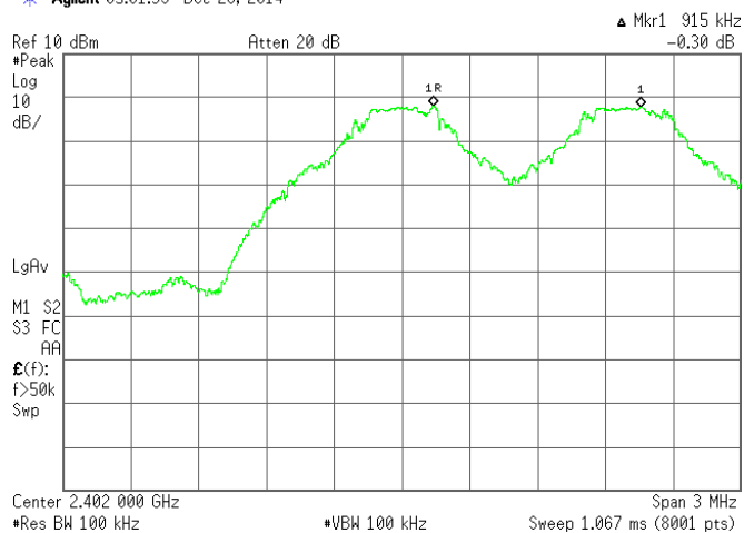
[BDR (DH3)]
