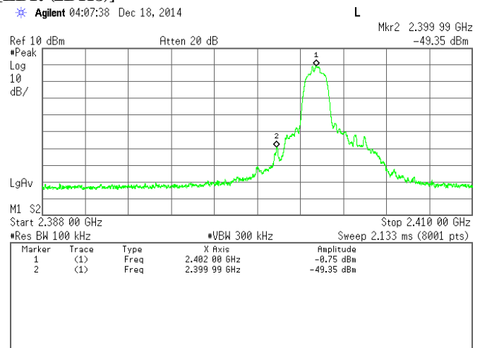
[EDR (2DH3)]
