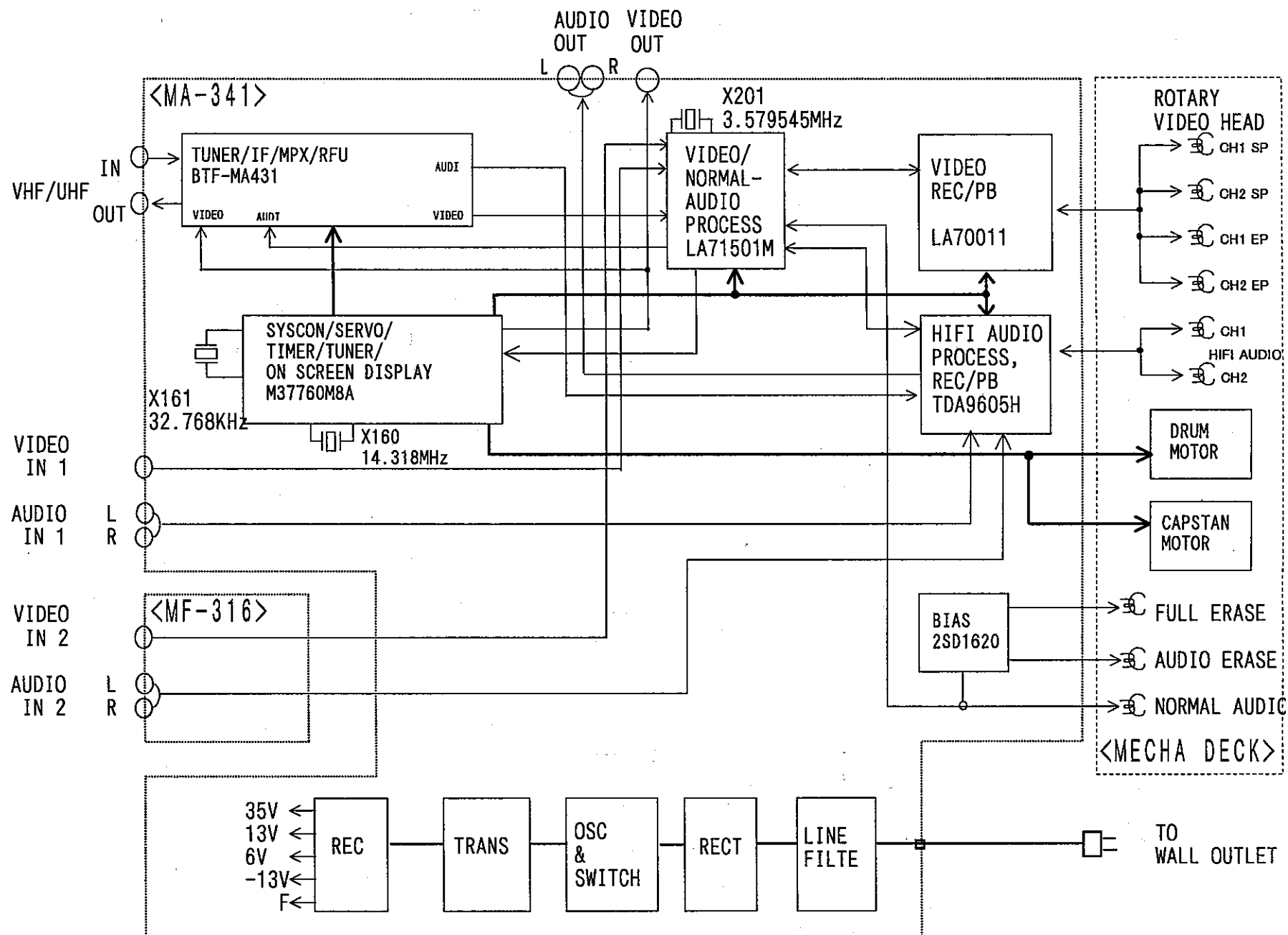
<<SLV-779HF BLOCK DIAGRAM>>
