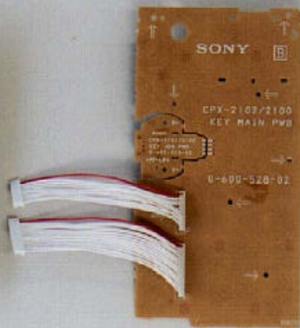
KEY PWB
