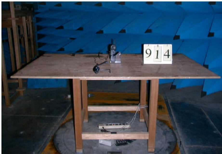
Picture 1 Front View of the Test Configuration (HANDSET)
