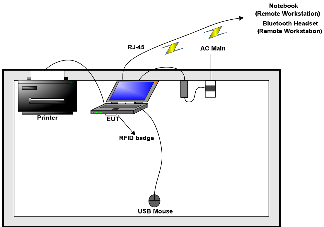
Test Setup Diagram - Radiated Above 1GHz Test
