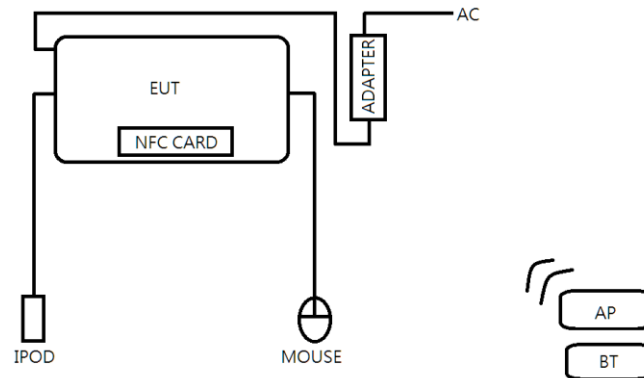
Test Setup Diagram – Radiated Emission Above 1GHz Test
