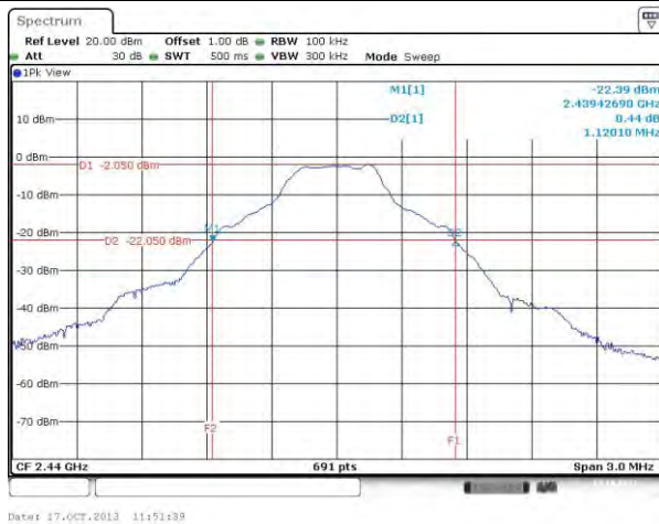
Worst 20dB Bandwidth Plots
