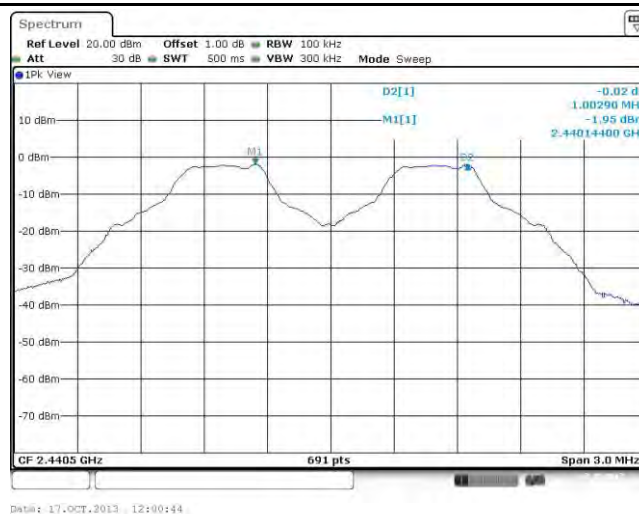
Worst Carrier Frequency Separation Plots
