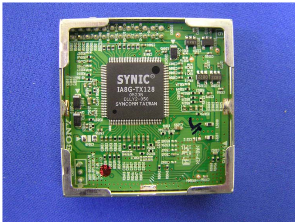
TX-RF Unit (Top)
