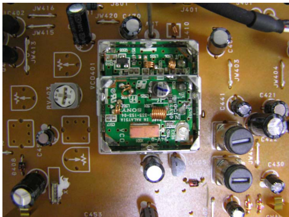
VCO Unit (Top)
