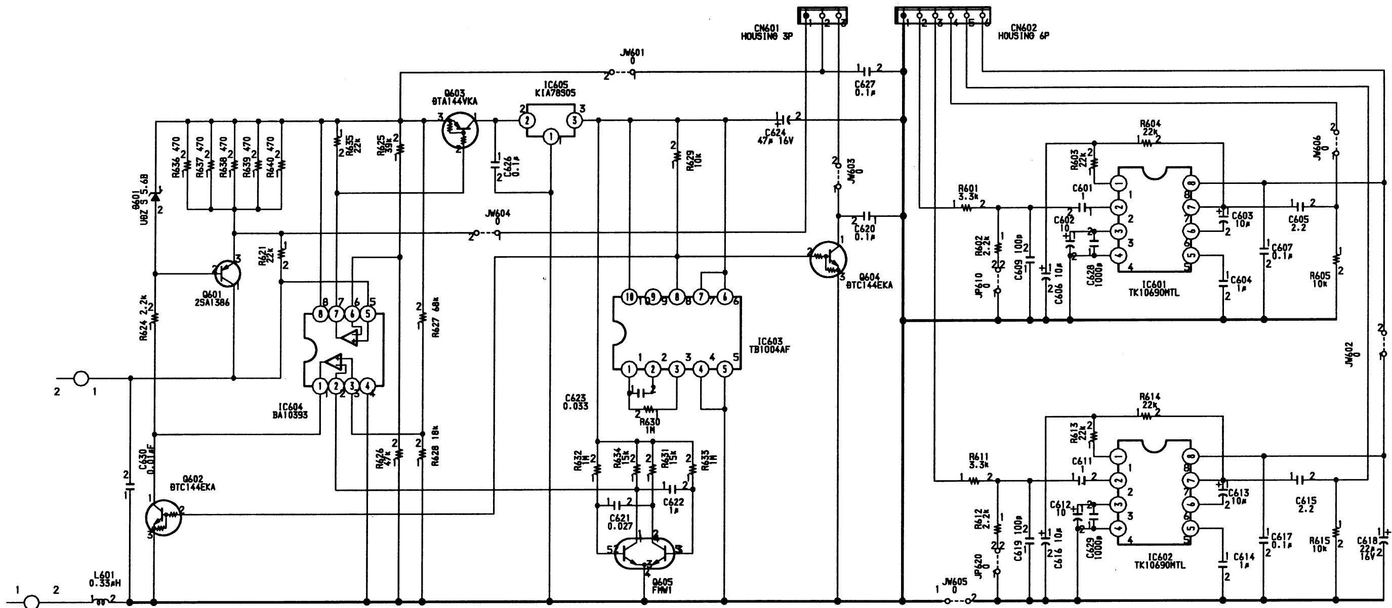
TMR-RF975R NR-CHG Circuit
