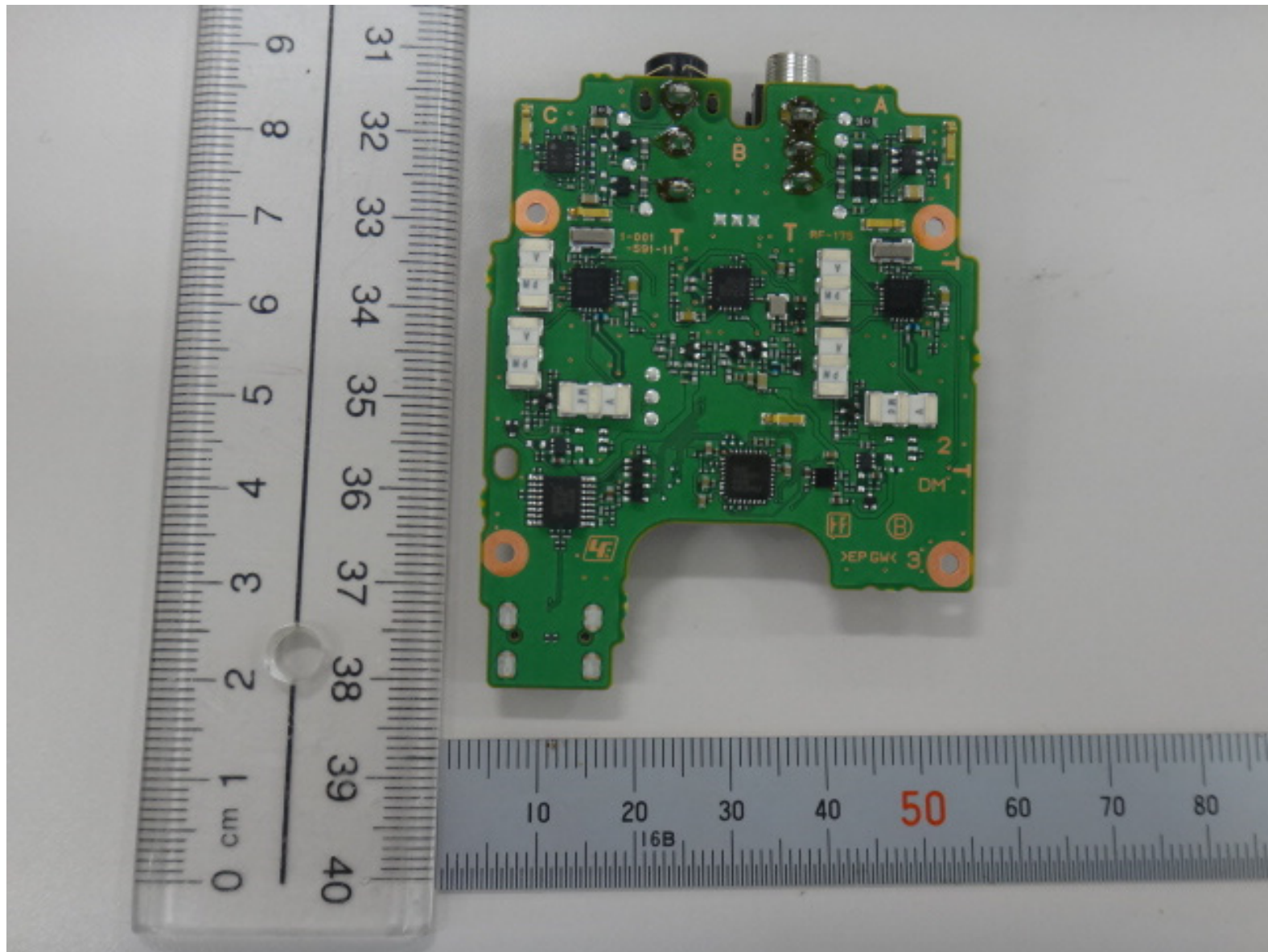
Side B of Board RF-175.
