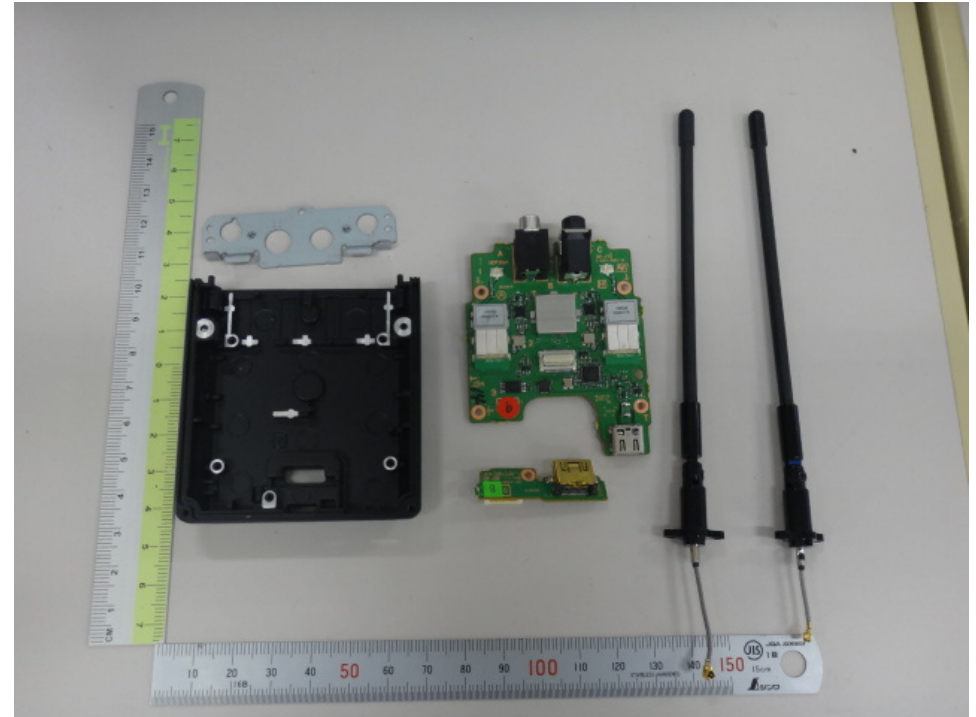
Rear Cabinet & RF-175,CN-4091
