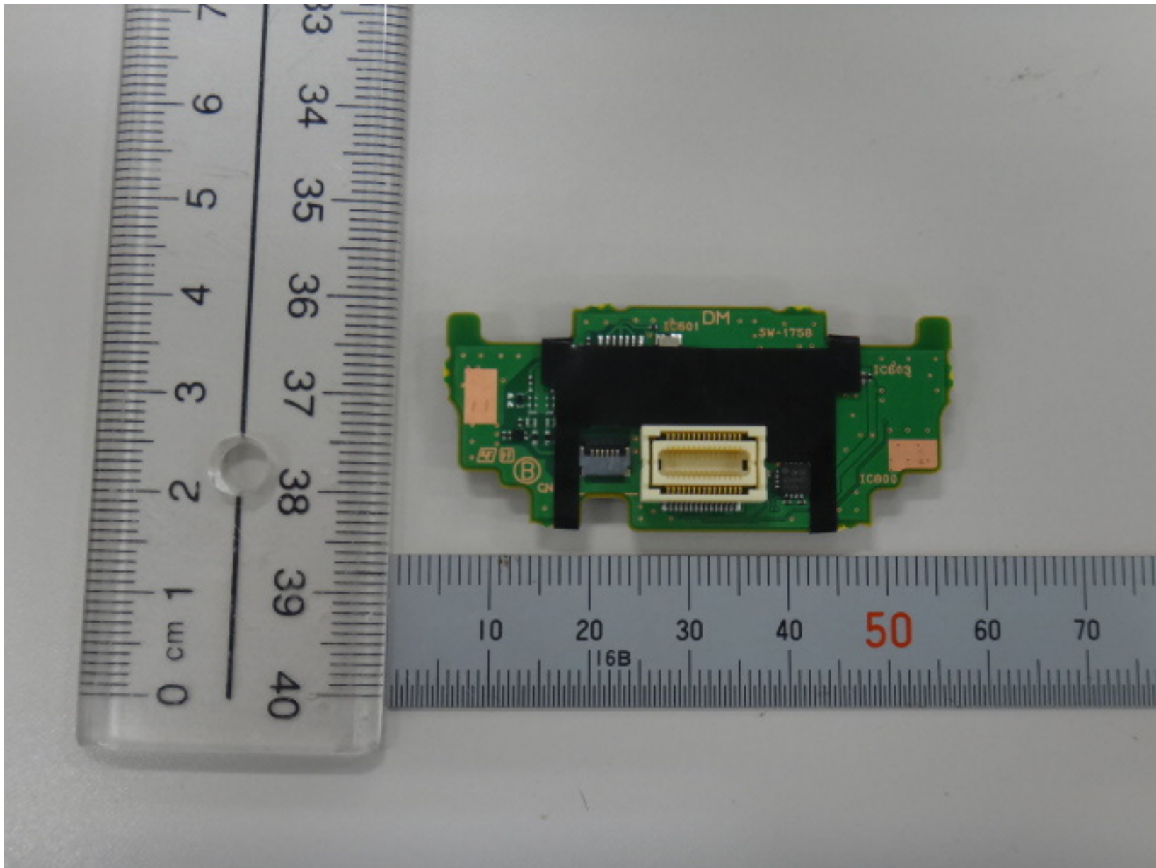
Side B of Board SW-1758.
