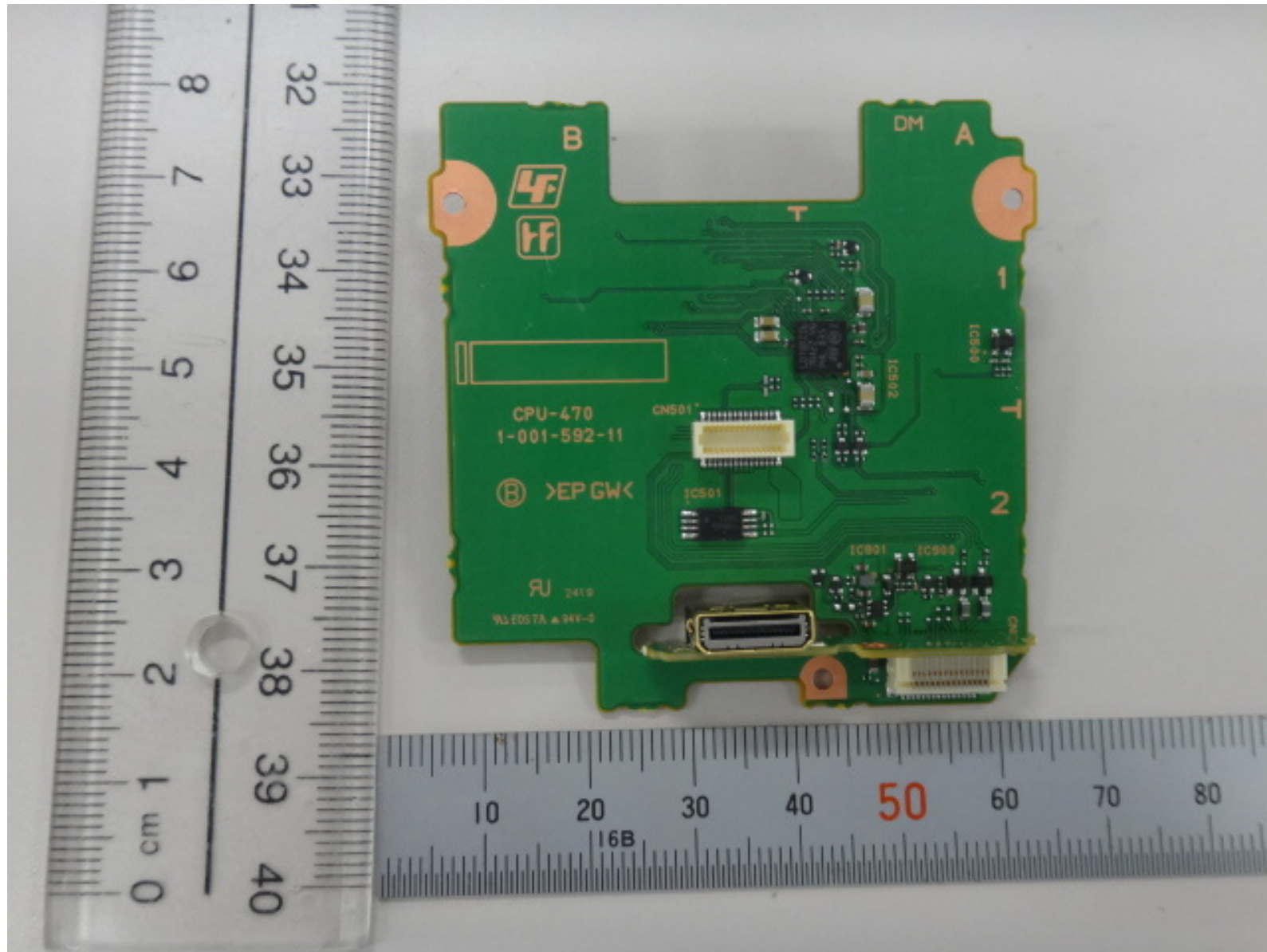
Side B of Board CPU-470.
