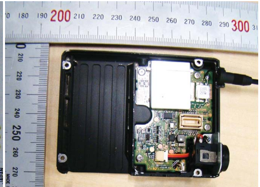
Rear Cabinet Side
