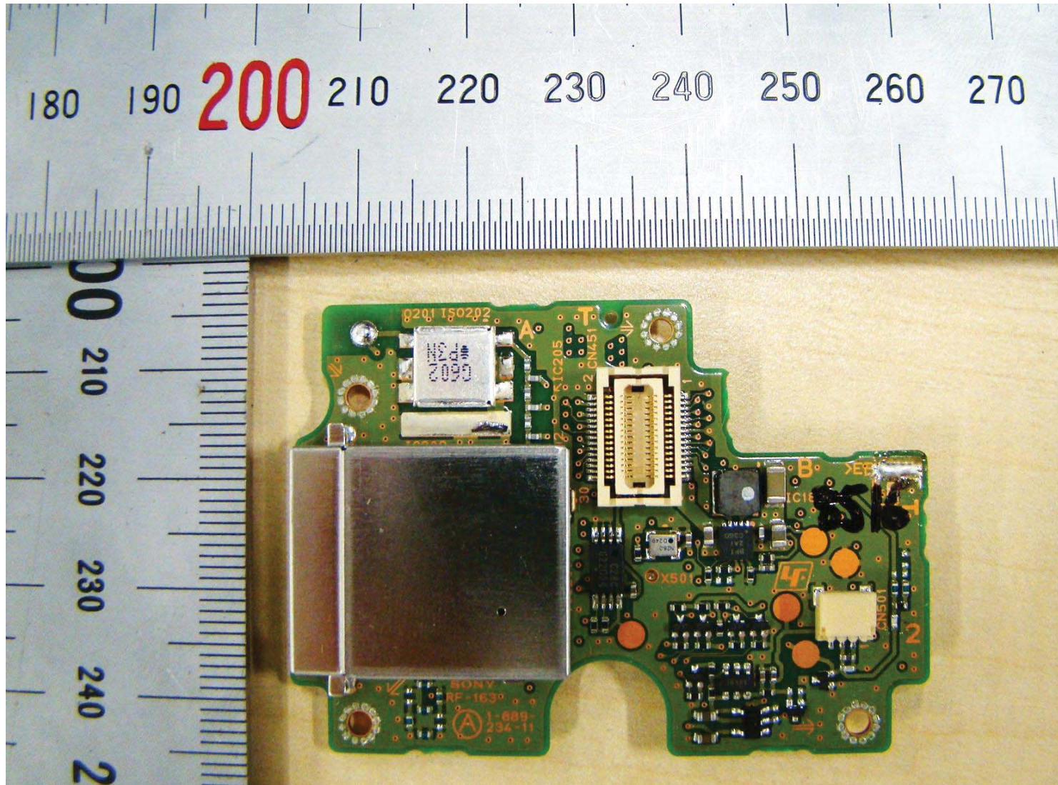
Side A of Board RF-163. (With Shield case)
