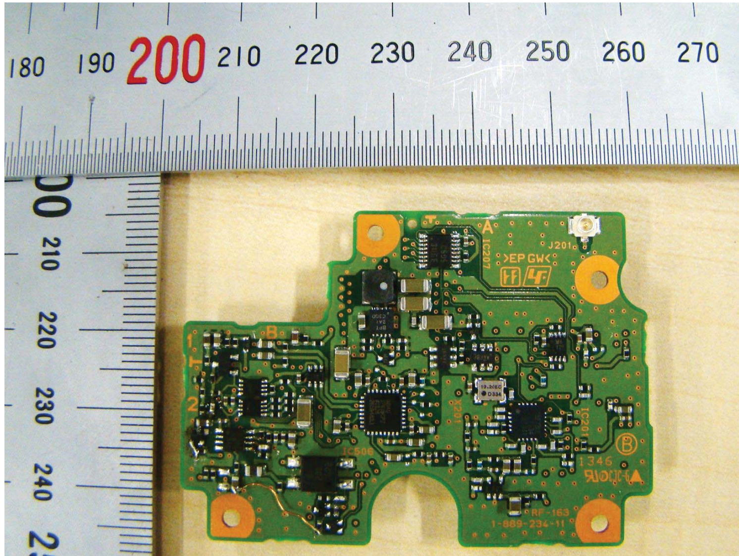
Side B of Board RF-163.
