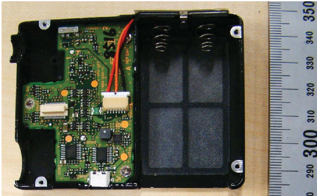
Front Cabinet Side
