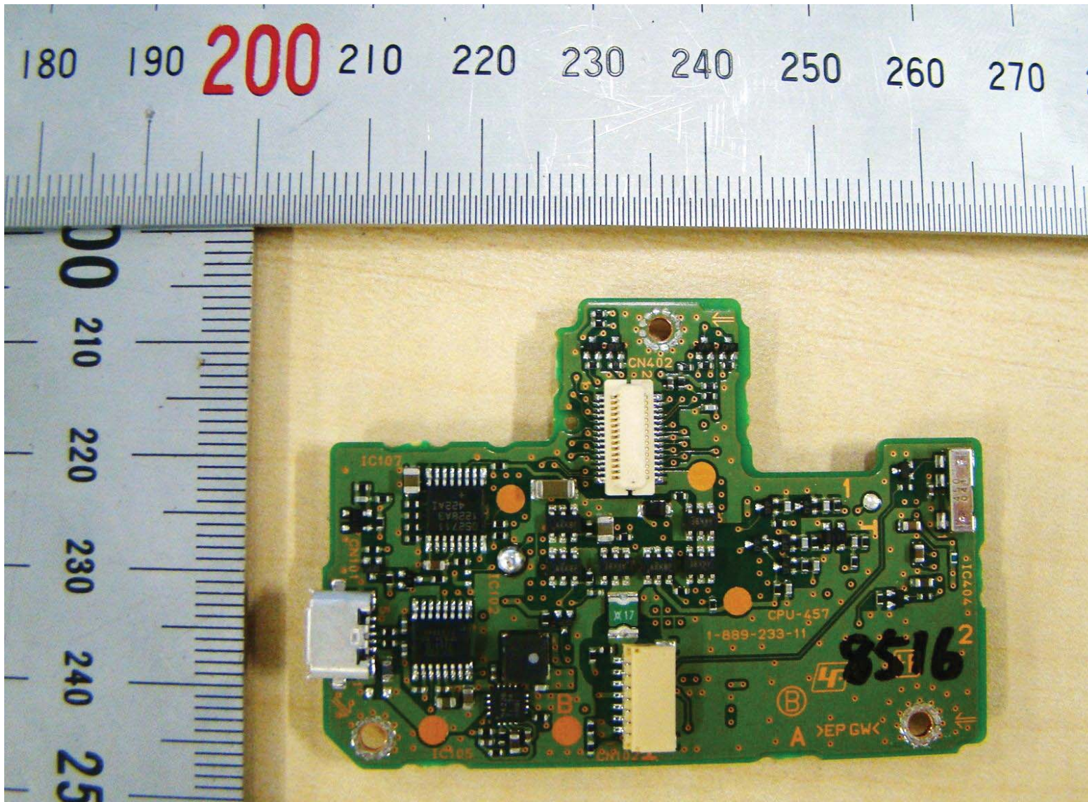
Side B of Board CPU-457.
