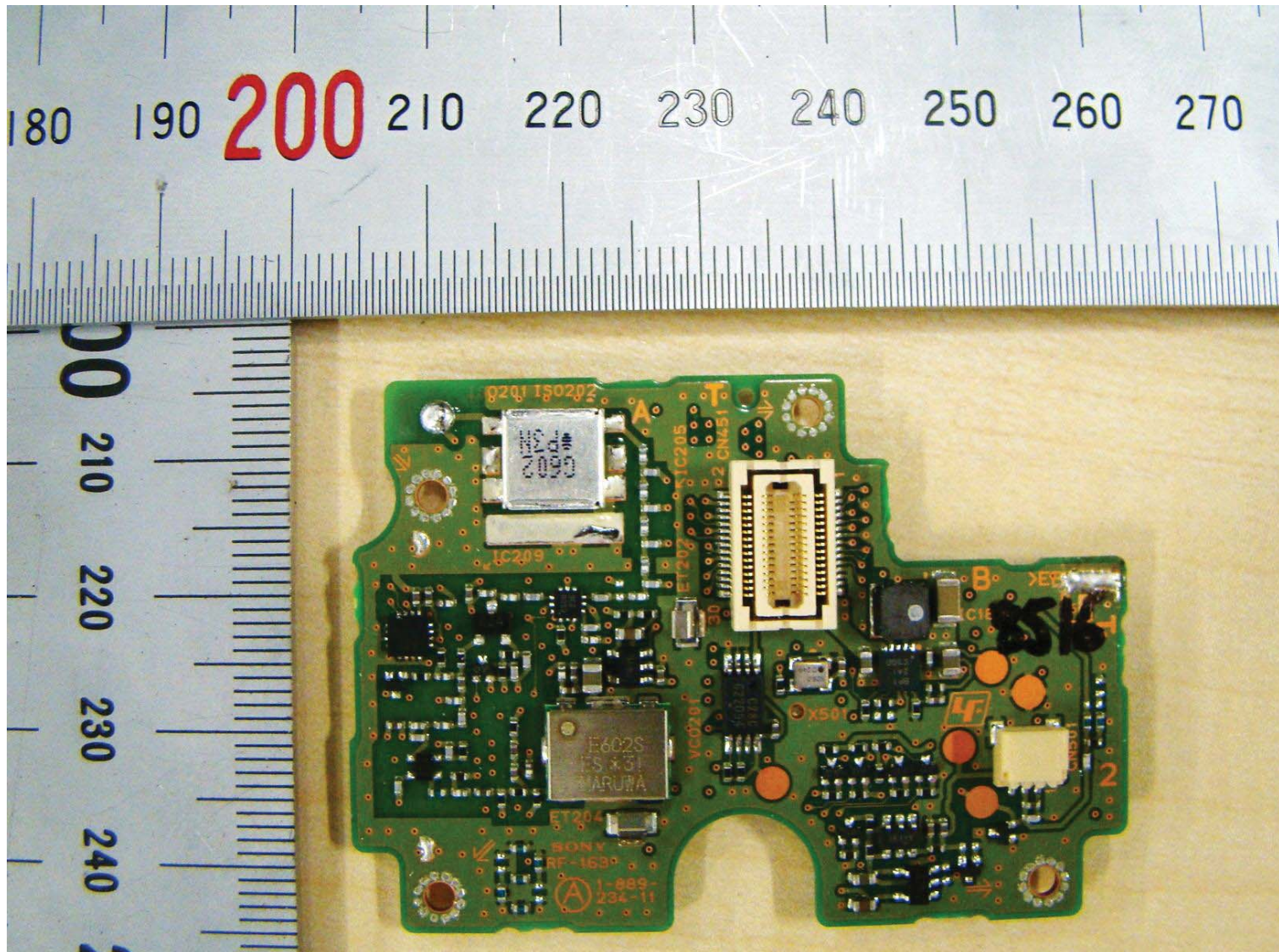
Side A of Board RF-163. (Without Shield case)
