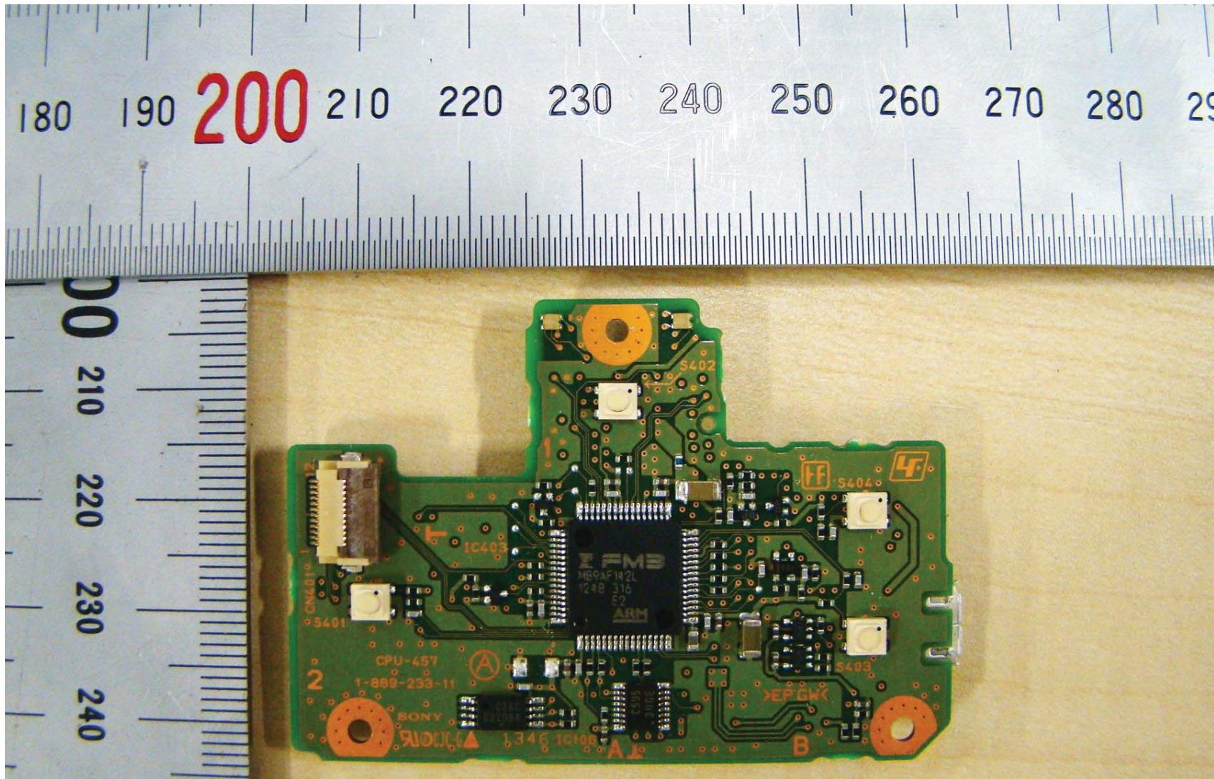
Side A of Board CPU-457.
