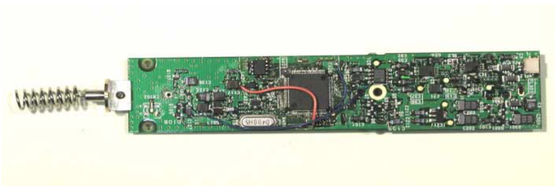
Photo-6: Inside PC Board, Face B
