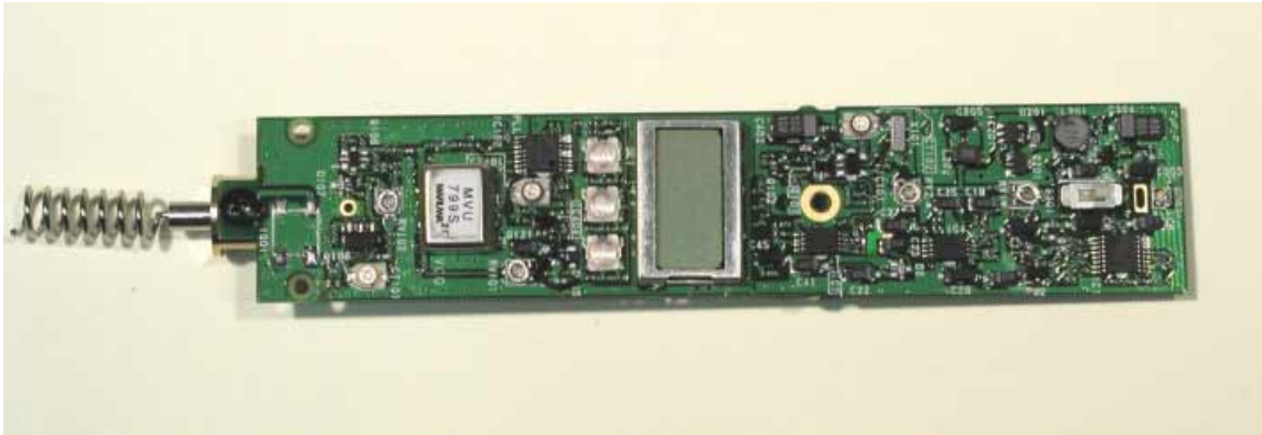
Photo-5: Inside PC Board, Face A
