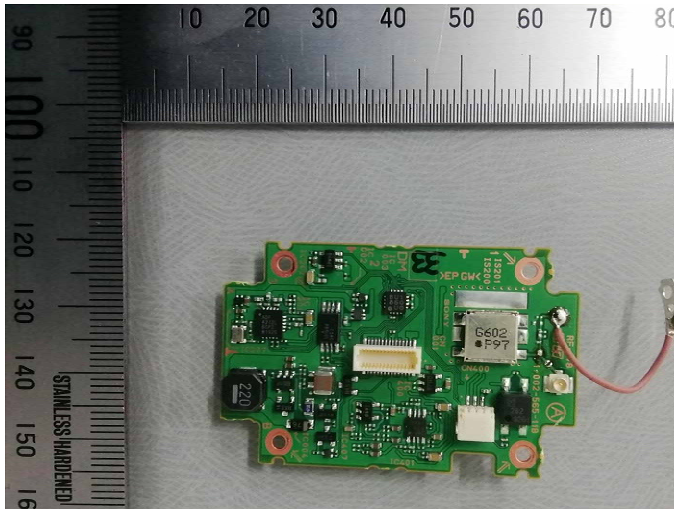
Side A of Board RF-178.
