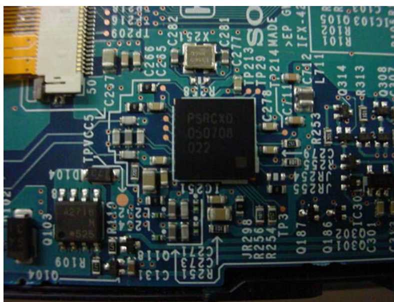
RF Circuit part (enlarged)
