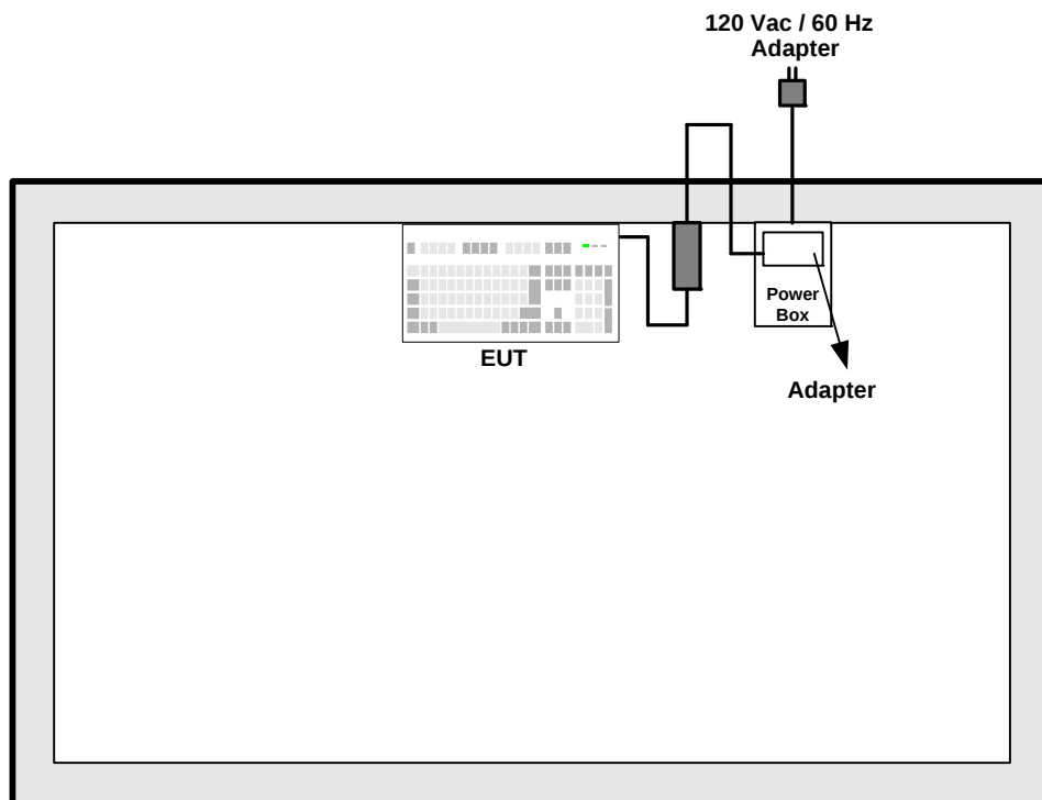
Test Setup Diagram - Radiated Test (Below 1GHz) Charge Mode
