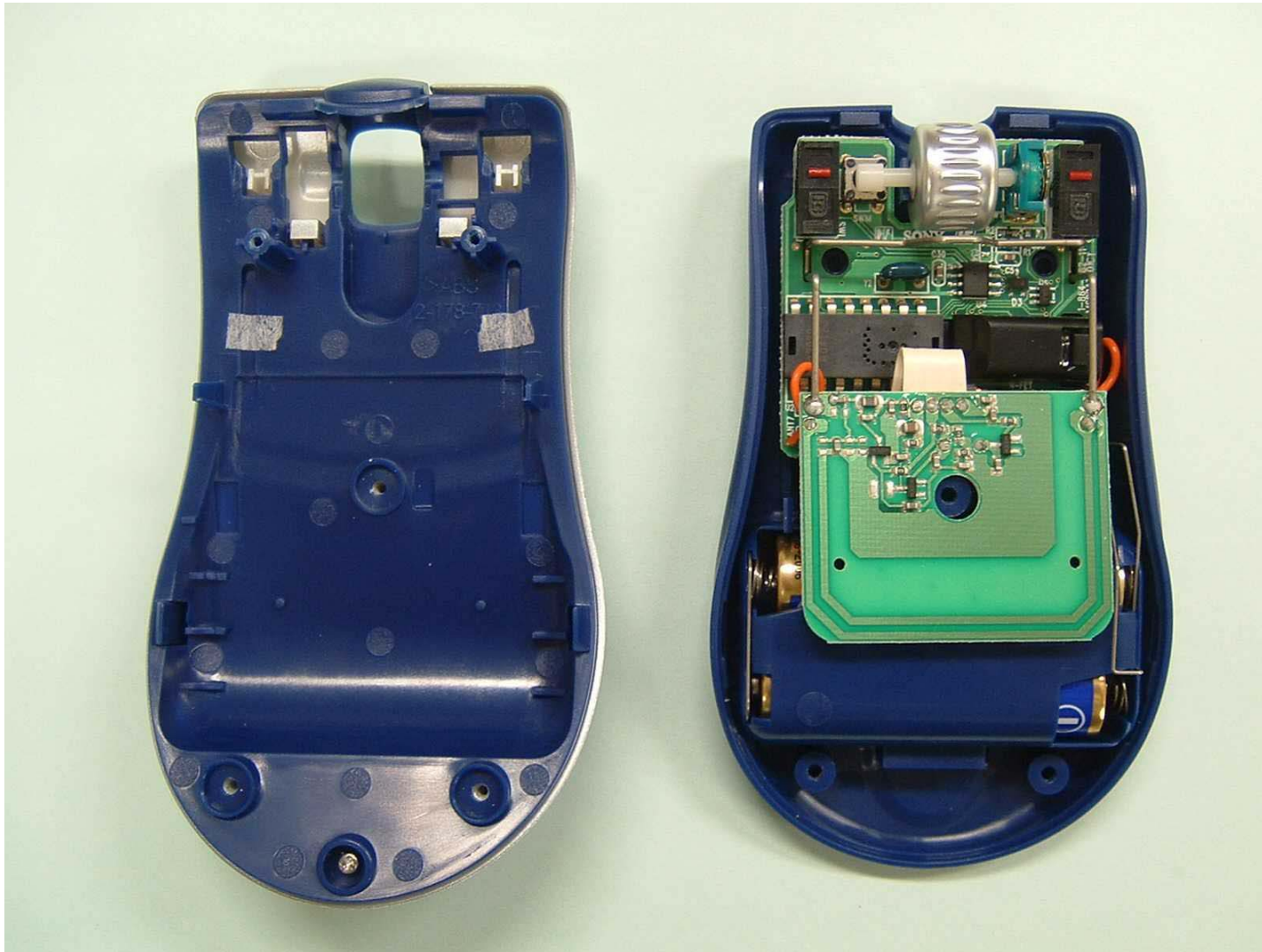
Cover Opened (SMU-WCL2)
