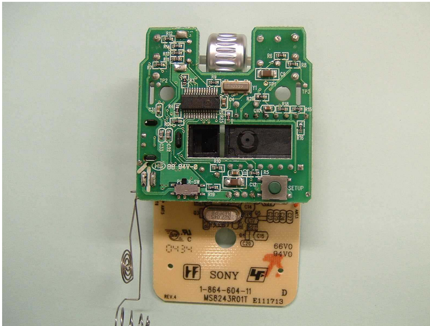
Rear Internal Circuit
