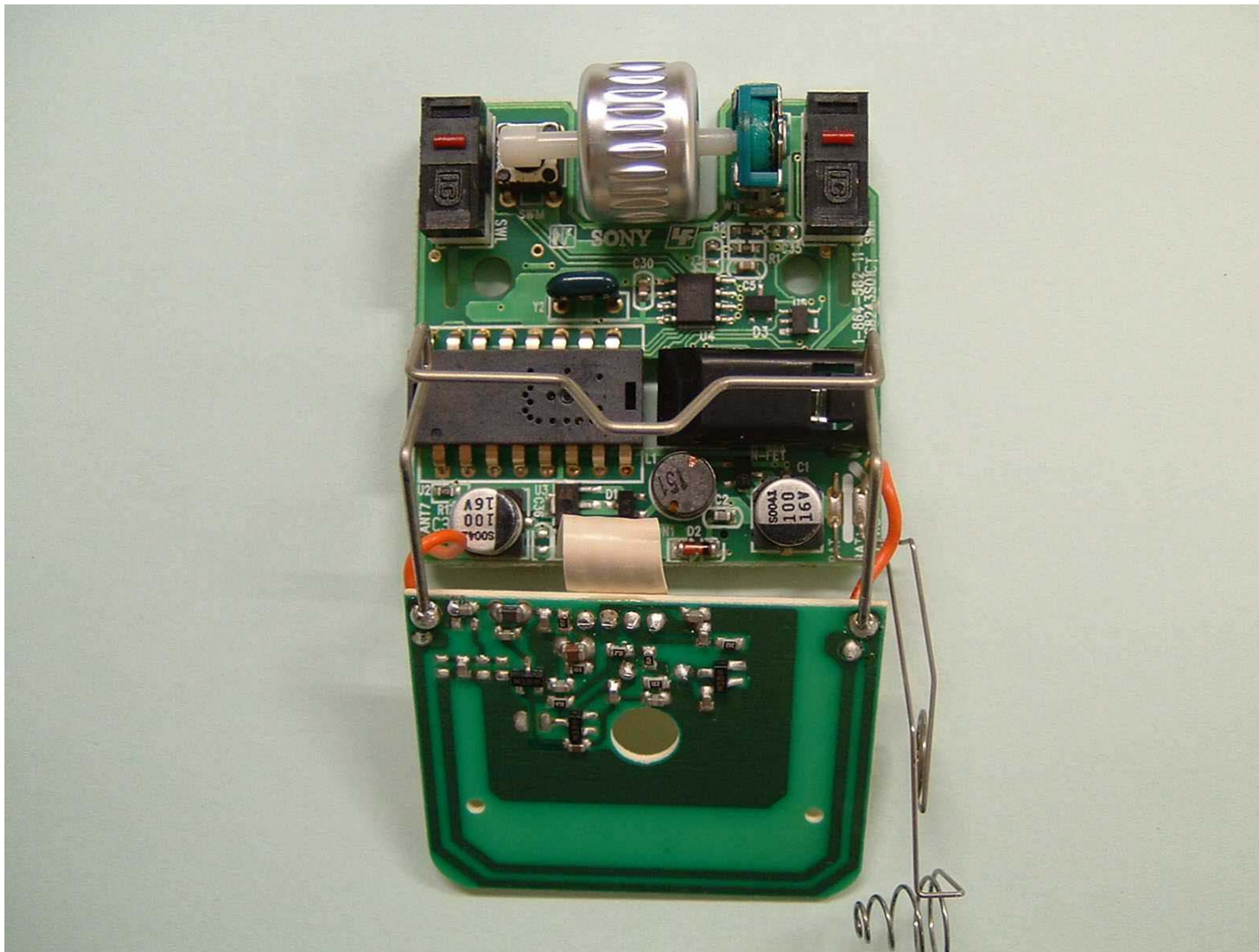
Front Internal Circuit
