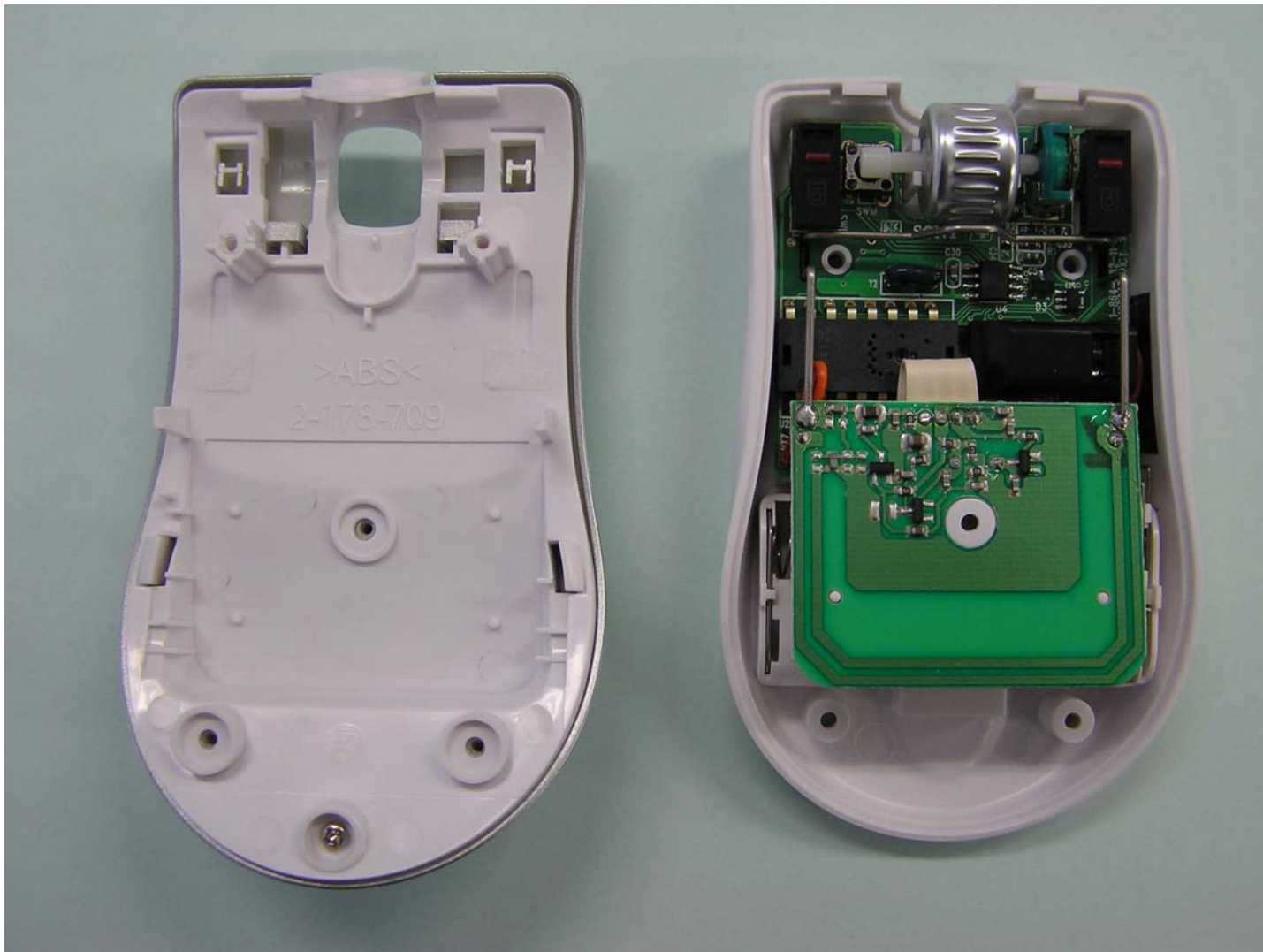
Cover Opened (SMU-WCM2)
