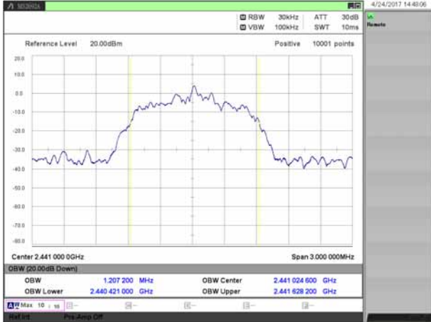
[EDR / 2441MHz]
