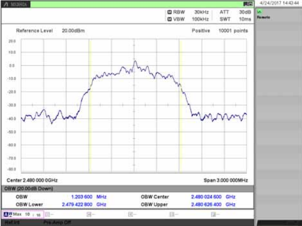
[EDR / 2480MHz]
