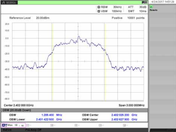
[EDR / 2402MHz]
