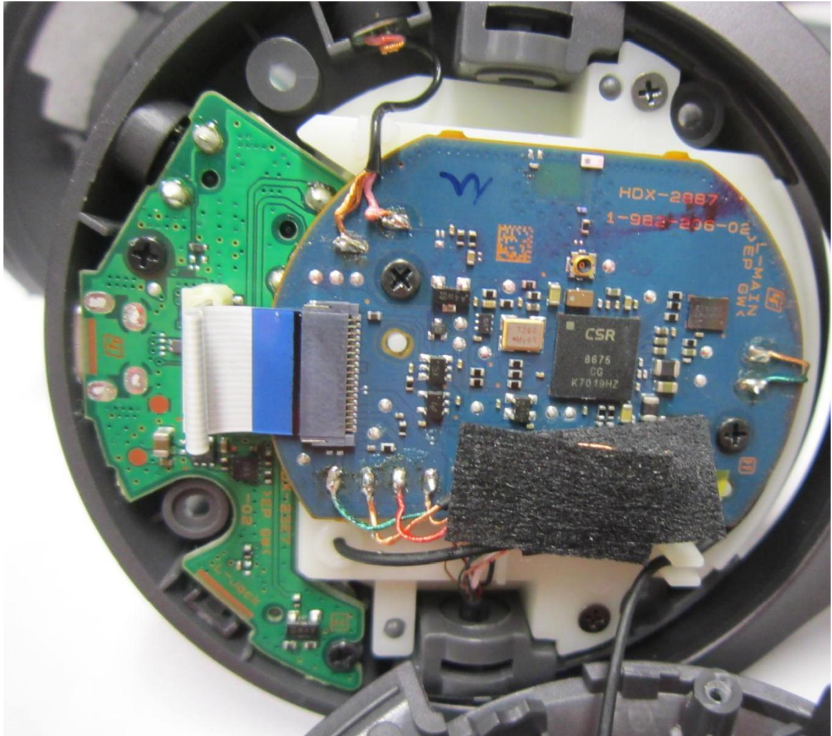
Left Side Headphone PCB Photo - Bottom
