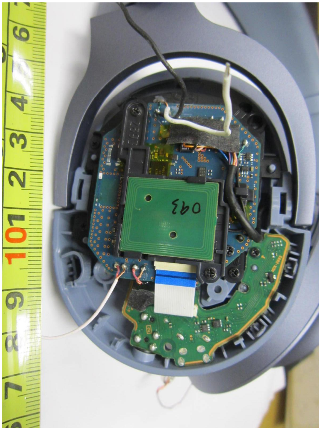
Left Side Headset Bottom
