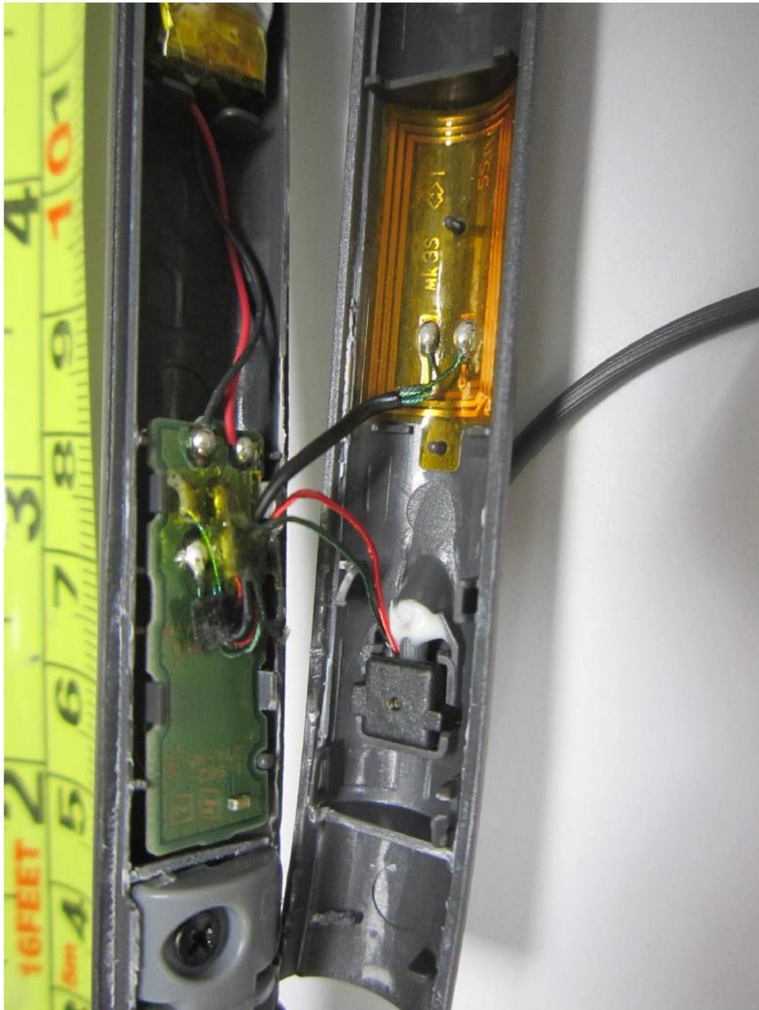
Right Side PCB Photo – (Close View)
