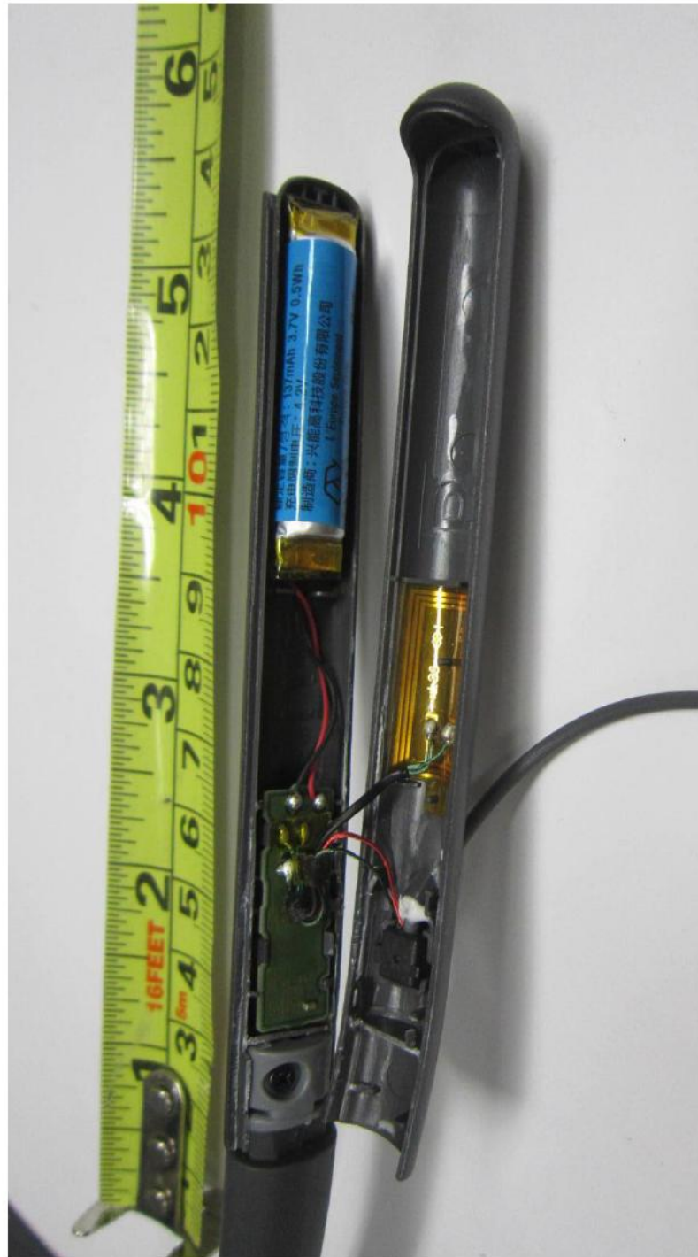
Right Side PCB Photo
