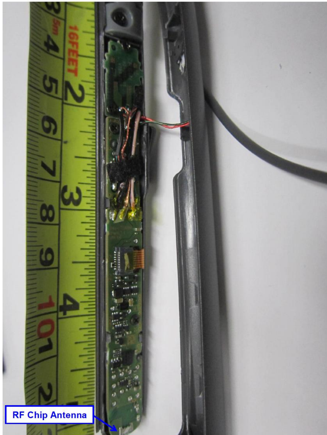
Left Side PCB Photo – (Close View)
