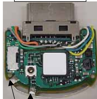
PWB, side B
