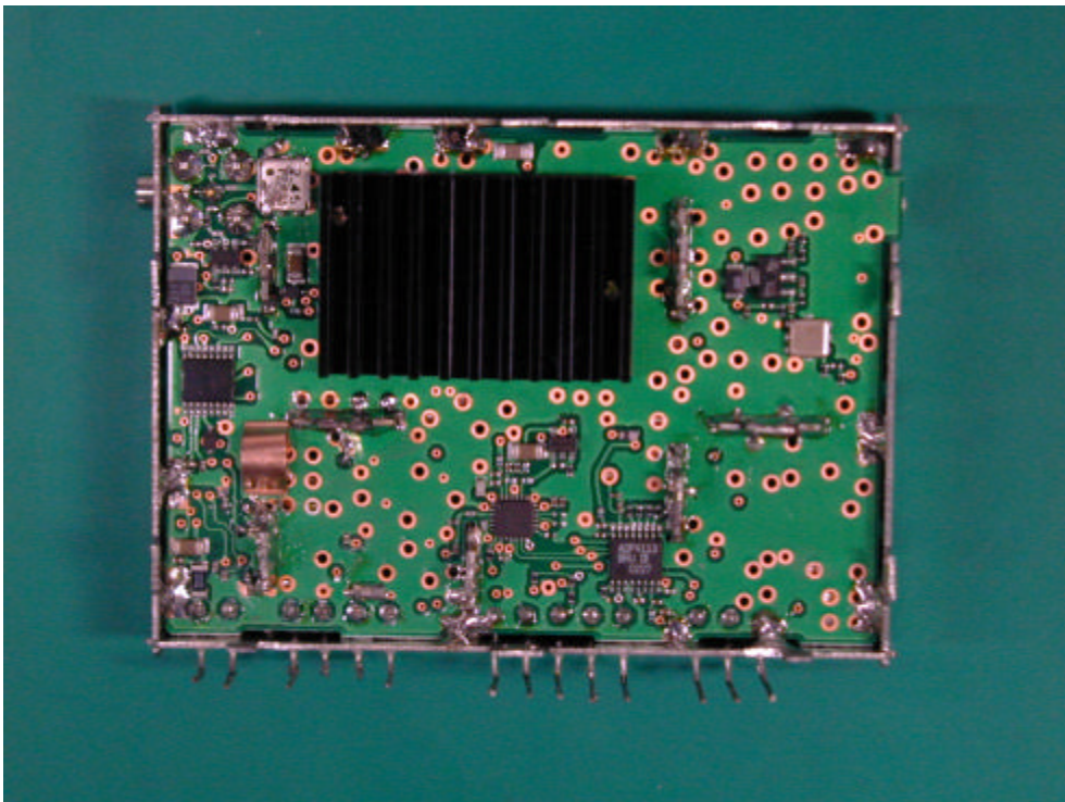
< Back side of RF Part without Shield >
