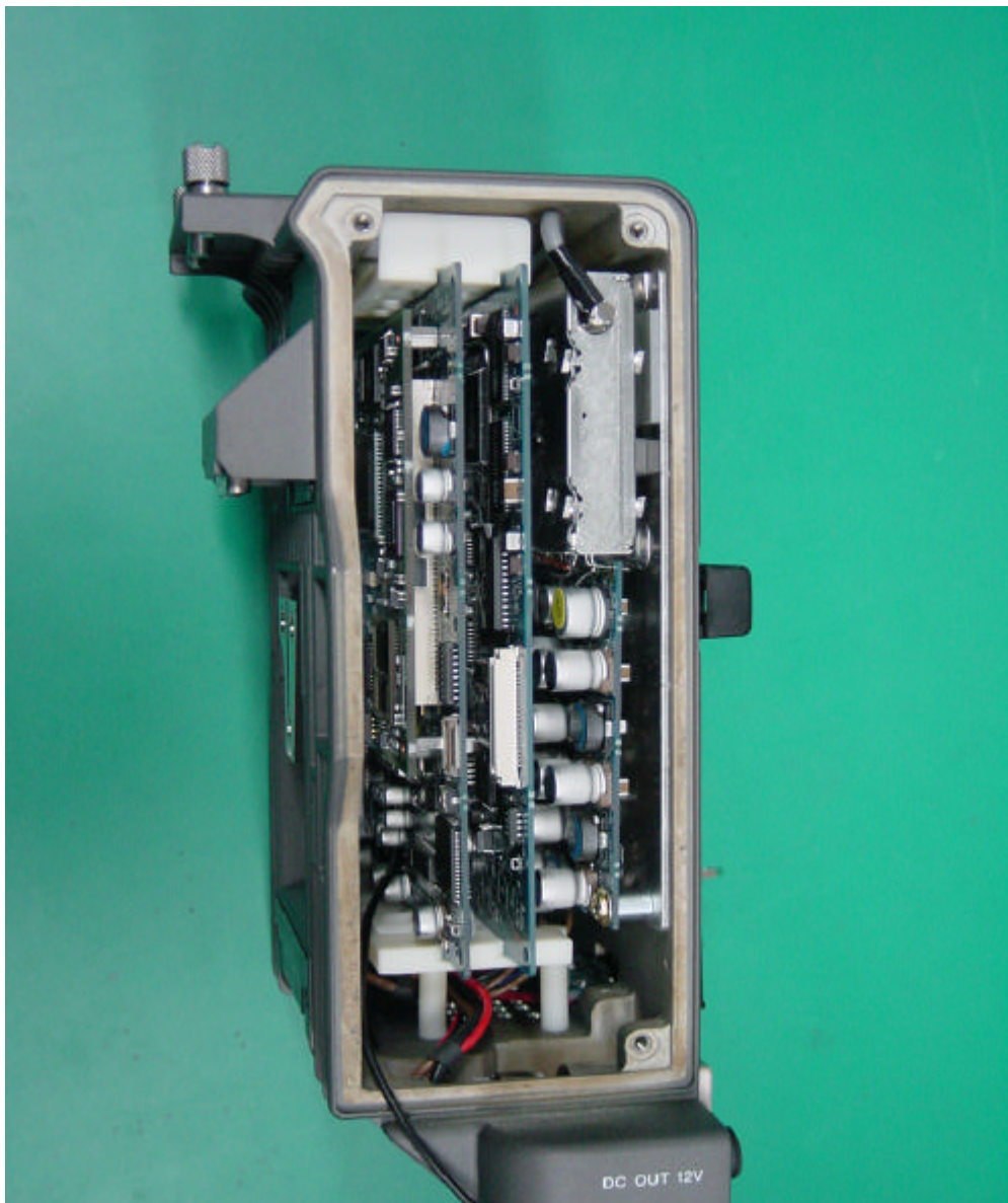
< Internal of Transmitter >
