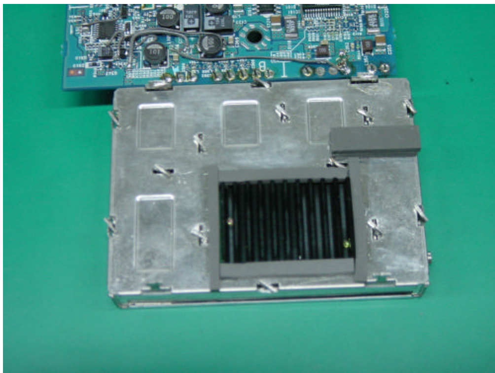
< Back side of RF Part with Shield >
