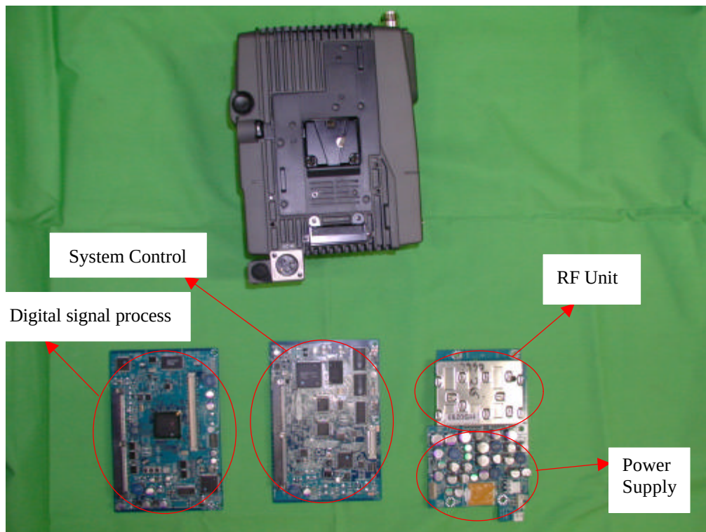
< Outside of Transmitter and Front side of PCB >
