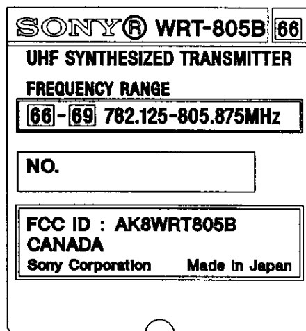
NAME PLATE
