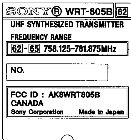
NAME PLATE
