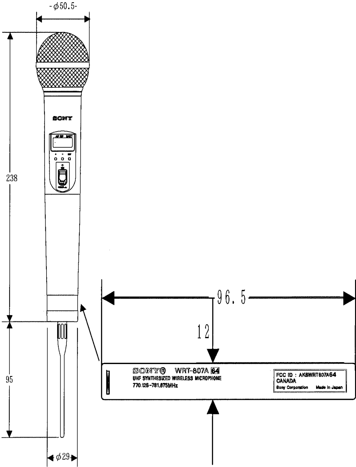
(f) Drawing of equipment identification plate.
