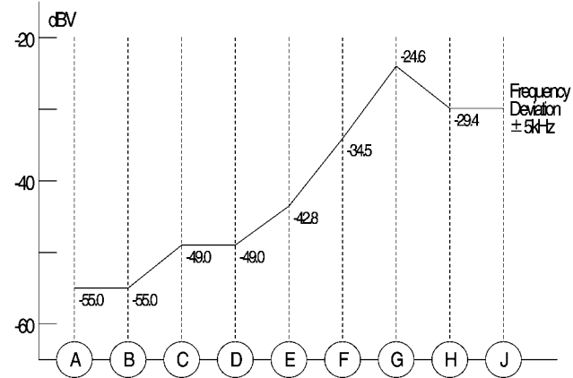
• LEVEL DIAGRAM
