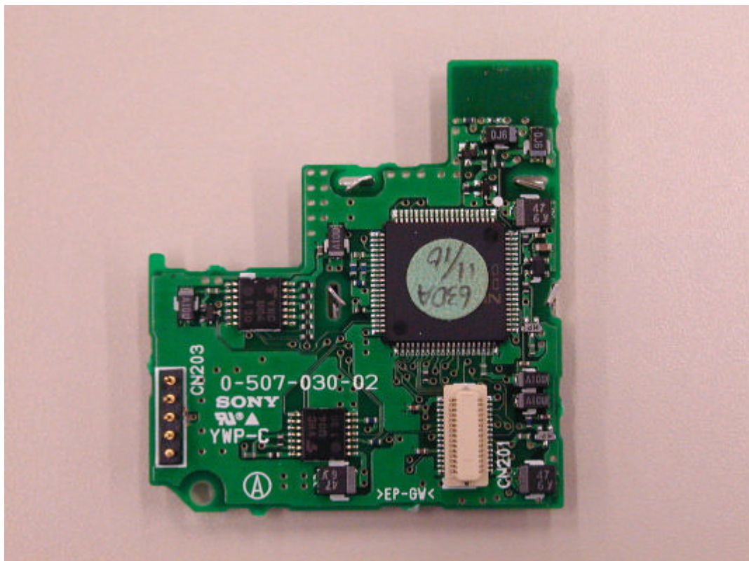
Circuit board 2
