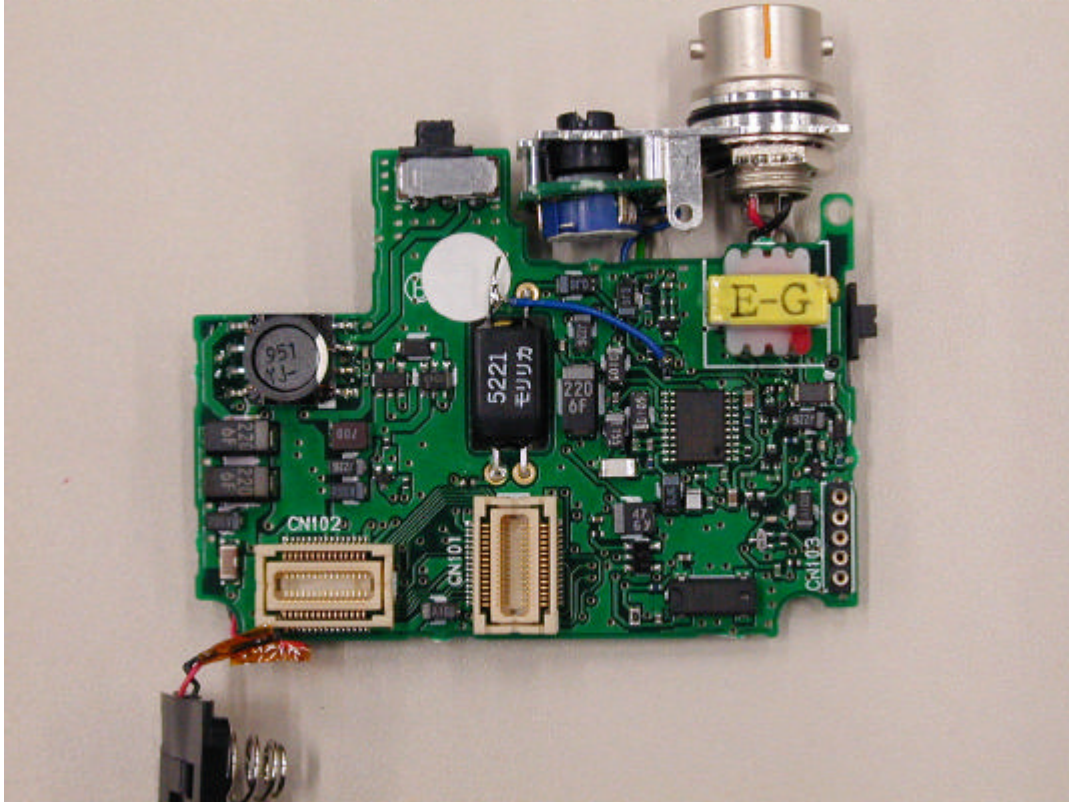
Circuit board 1
