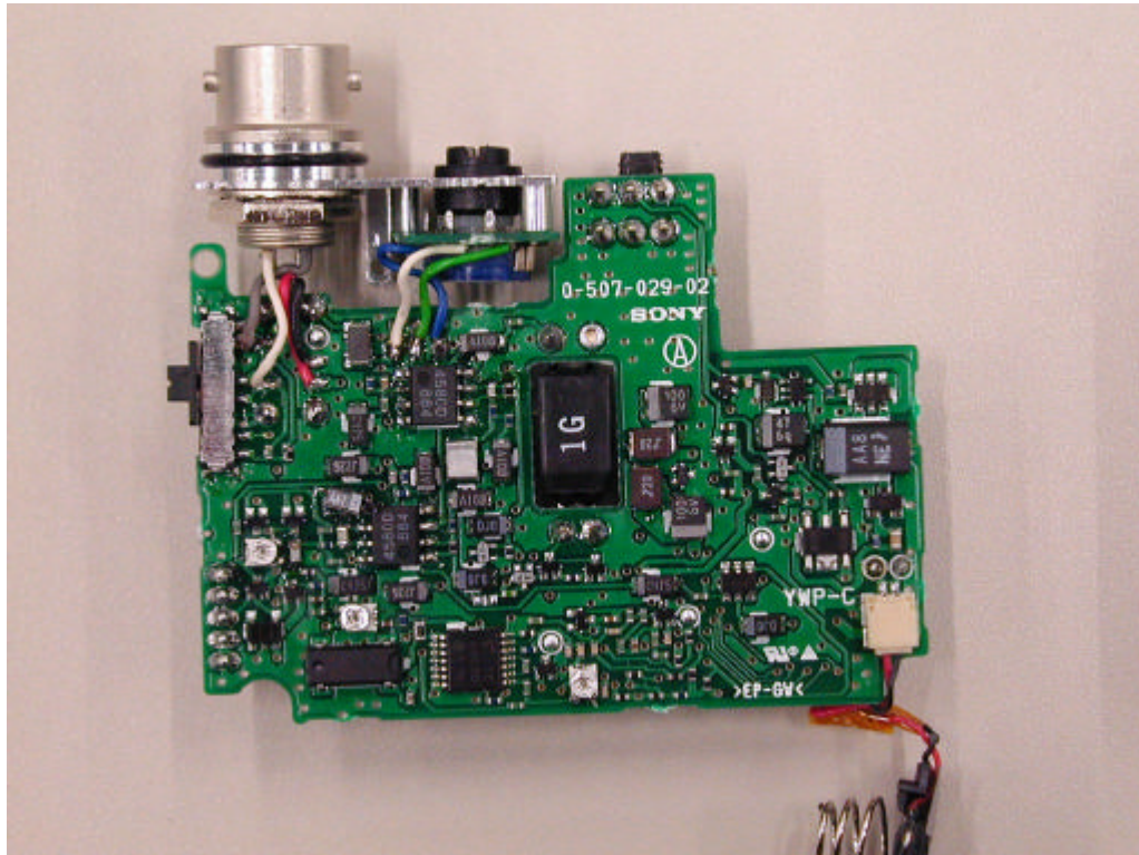
Circuit board 1
