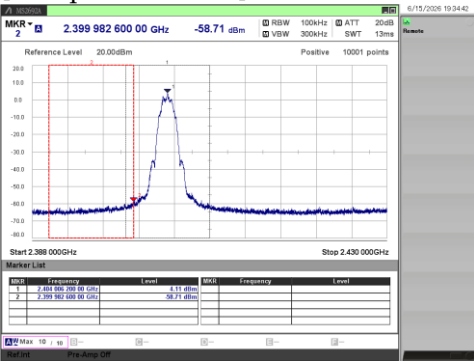
[2 Mbps / 2404 MHz]
