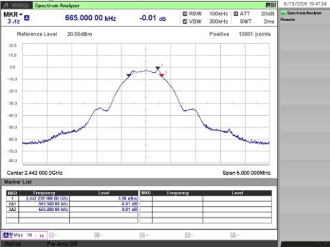
[1 Mbps / 2442 MHz]
