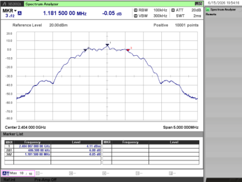
[2 Mbps / 2404 MHz]
