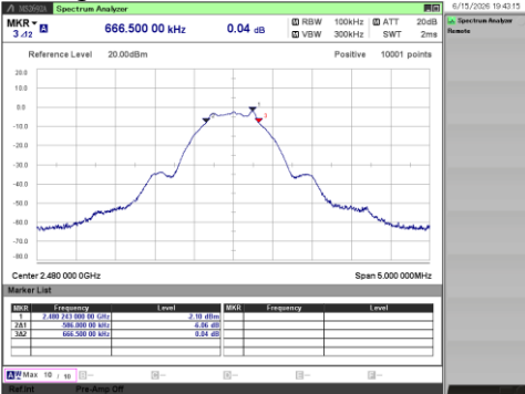
[1 Mbps / 2480 MHz]
