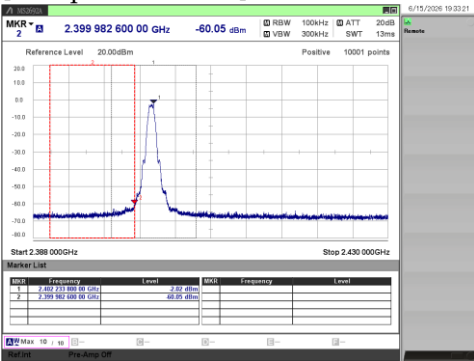
[1 Mbps / 2402 MHz]
