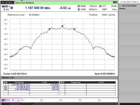
[2 Mbps / 2442 MHz]
