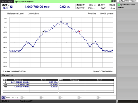
[BDR / 2480 MHz]
