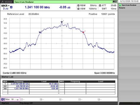
[EDR / 2480 MHz]
