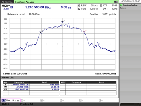
[EDR / 2441 MHz]
