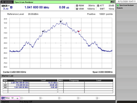
[BDR / 2402 MHz]
