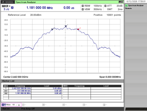
[ 2 Mbps / 2442 MHz]
