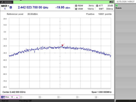
[1 Mbps / 2442 MHz]
