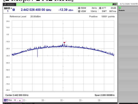
[2 Mbps / 2442 MHz]
