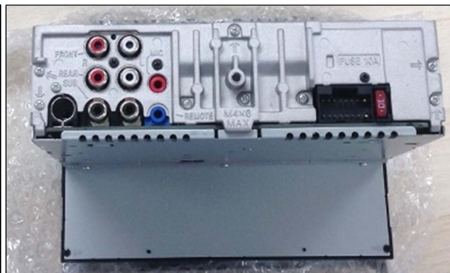
BACK SIDE
