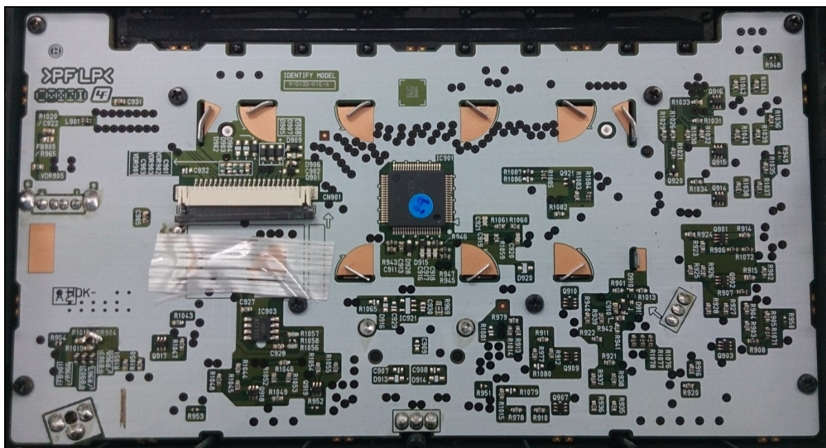
Back Side
