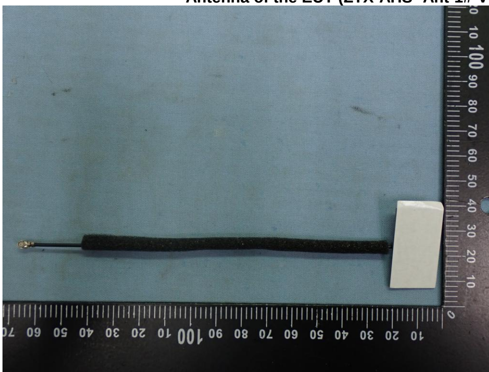
Figure 36 Antenna of the EUT (ZTX-AHS- Ant-1#-V03 (WIFI0) )
