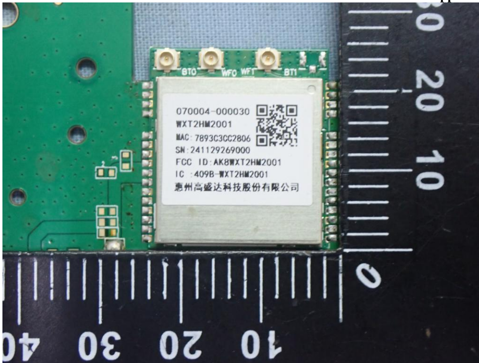
Figure 7 General Appearance of the EUT
