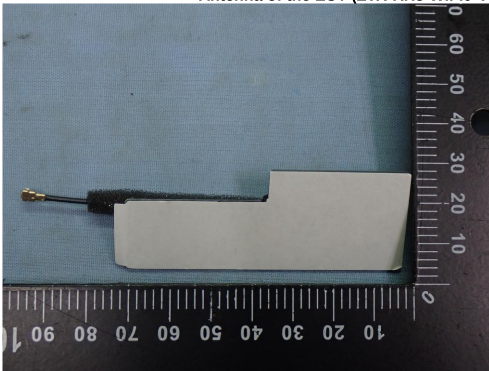
Figure 27 Antenna of the EUT (ZTX-RH5-WIFI0-V04 (WIFI0) )
