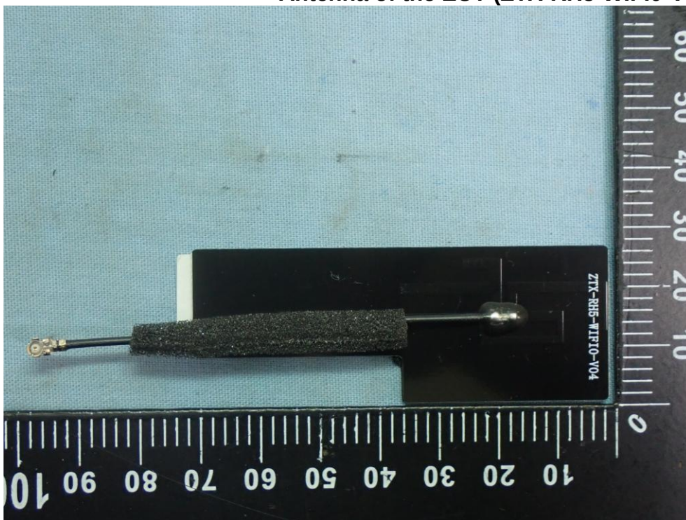
Figure 26 Antenna of the EUT (ZTX-RH5-WIFI0-V04 (WIFI0) )
