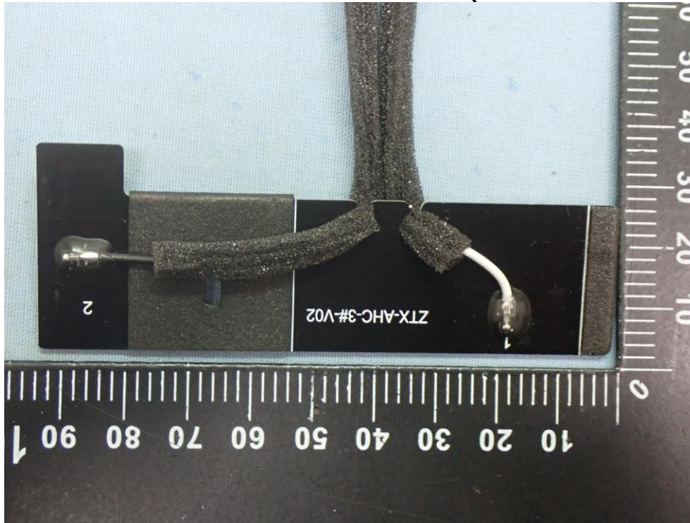
Figure 19 Antenna of the EUT (ZTX-AHC- Ant-3#-V02 (WIFI 0) )
