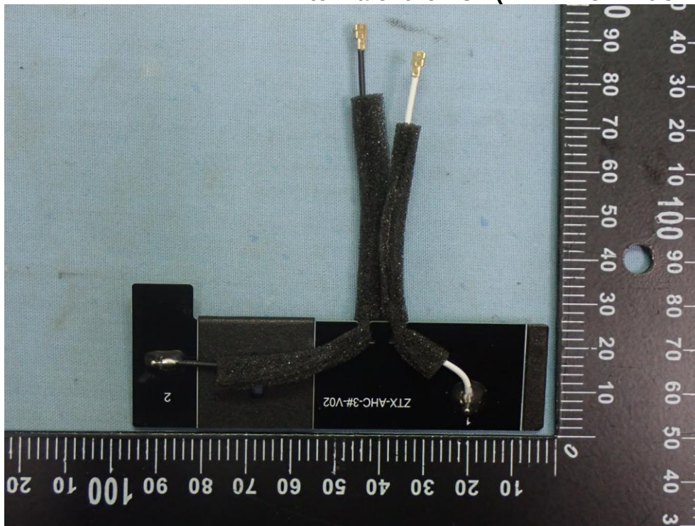
Figure 20 Antenna of the EUT (ZTX-AHC- Ant-3#-V02 (WIFI 1) )
