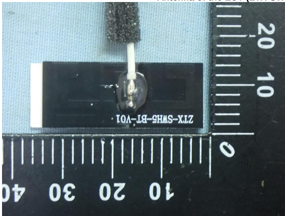
Figure 59 Antenna of the EUT (ZTX-SWH5-BT-V01)
