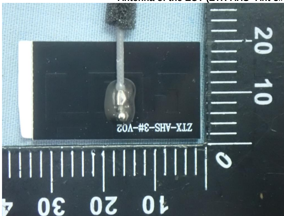
Figure 40 Antenna of the EUT (ZTX-AHS- Ant-3#-V02 (WIFI0) )
