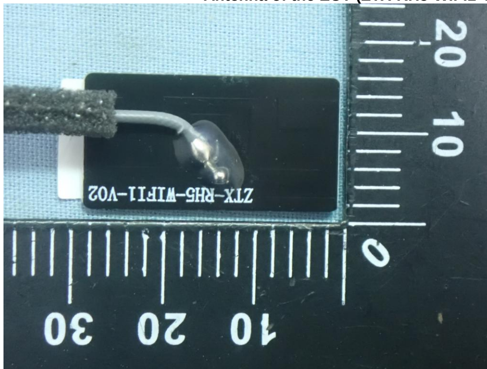
Figure 31 Antenna of the EUT (ZTX-RH5-WIFI1-V02 (WIFI1))
