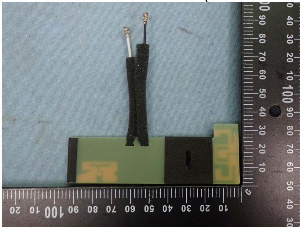
Figure 21 Antenna of the EUT (ZTX-AHC- Ant-3#-V02 (WIFI 1) )
