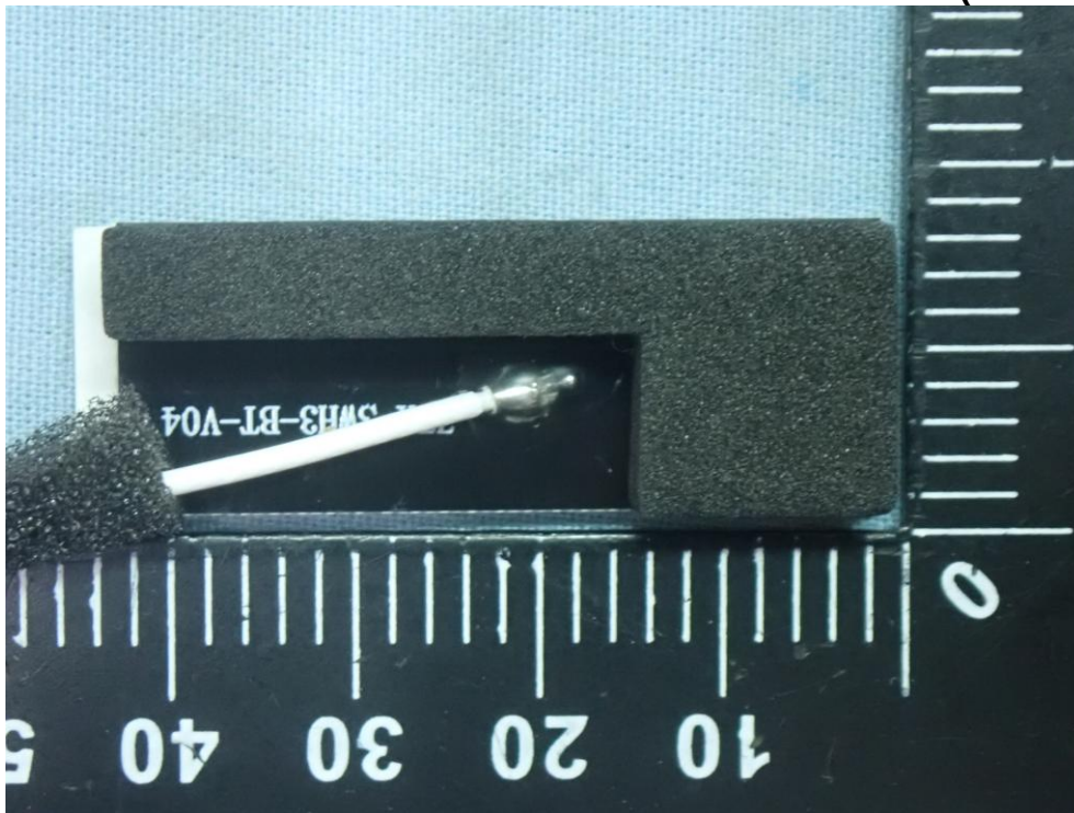
Figure 49 Antenna of the EUT (ZTX-SWH3-BT-V04)
