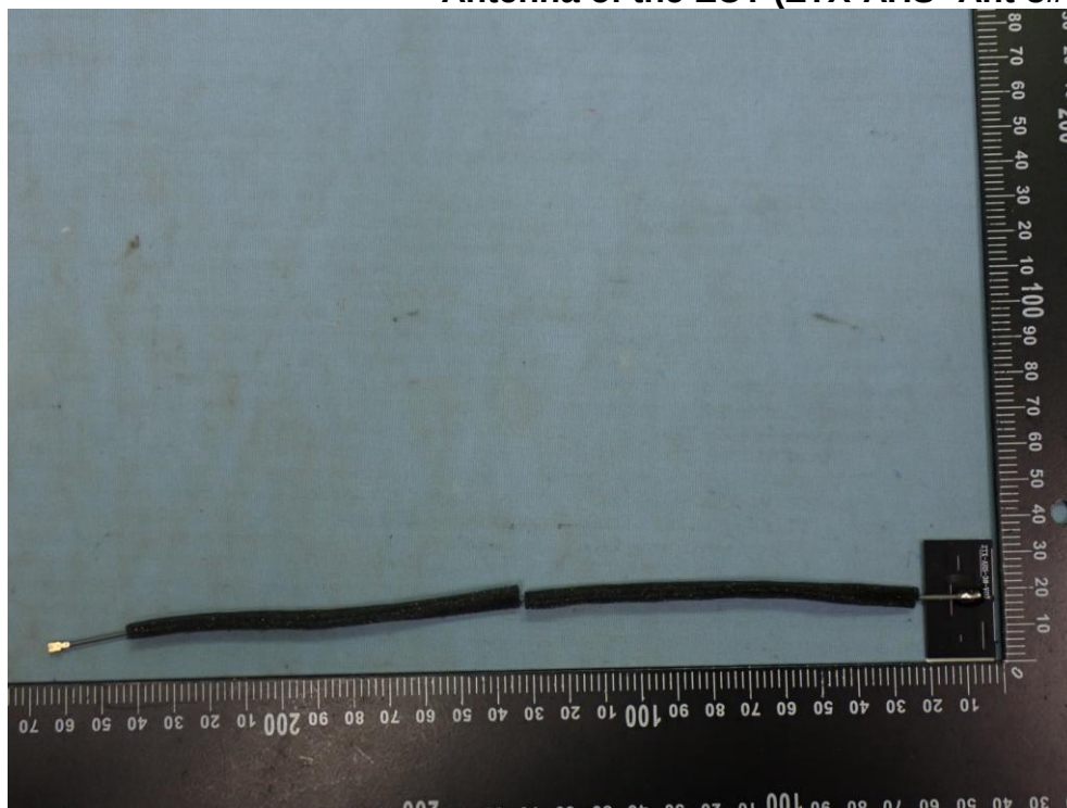
Figure 38 Antenna of the EUT (ZTX-AHS- Ant-3#-V02 (WIFI0) )
