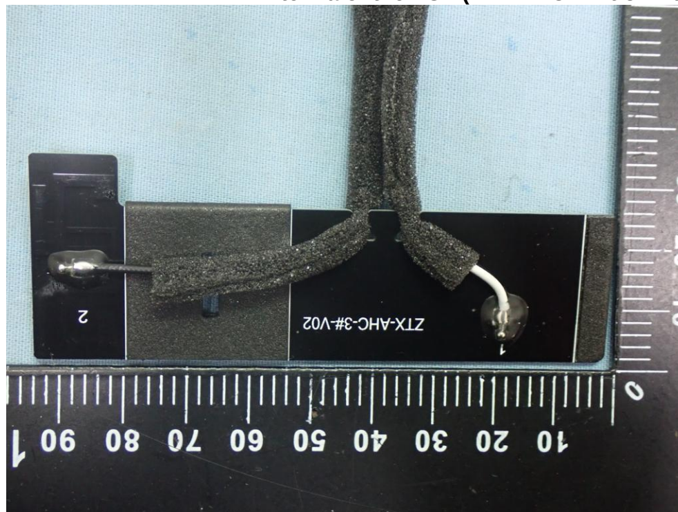
Figure 22 Antenna of the EUT (ZTX-AHC- Ant-3#-V02 (WIFI 1) )
