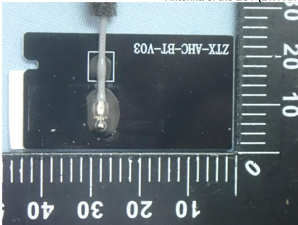
Figure 25 Antenna of the EUT (ZTX-AHC-BT -V03 )
