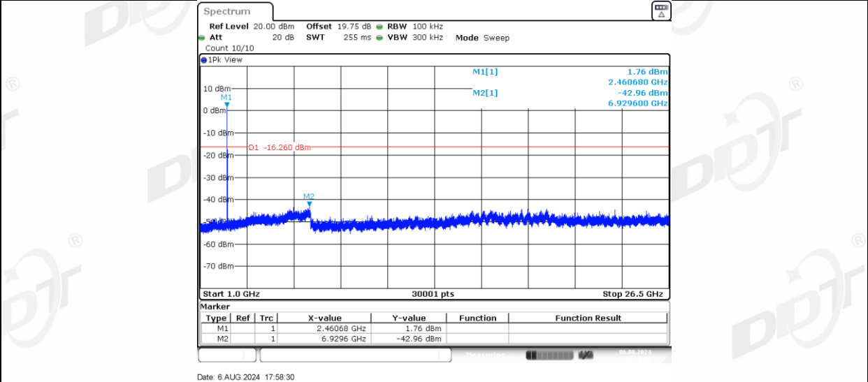
11B-CDD_Ant-3_2462_0~Reference
