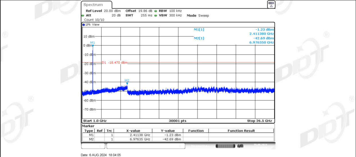
11G-CDD Ant-3_2412_0~Reference
