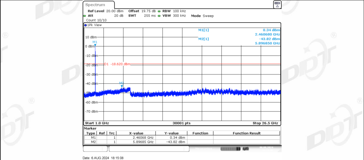
11G-CDD Ant-3_2462_0~Reference
