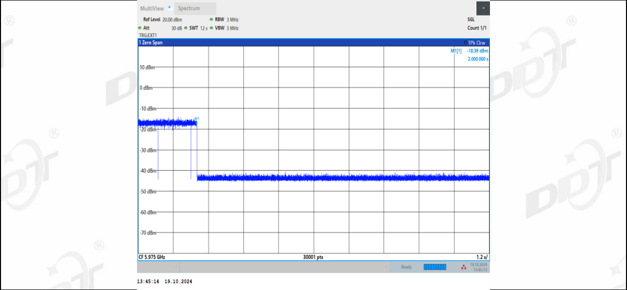
11AX20MIMO Ant1_5975_Center_5975_OFF
