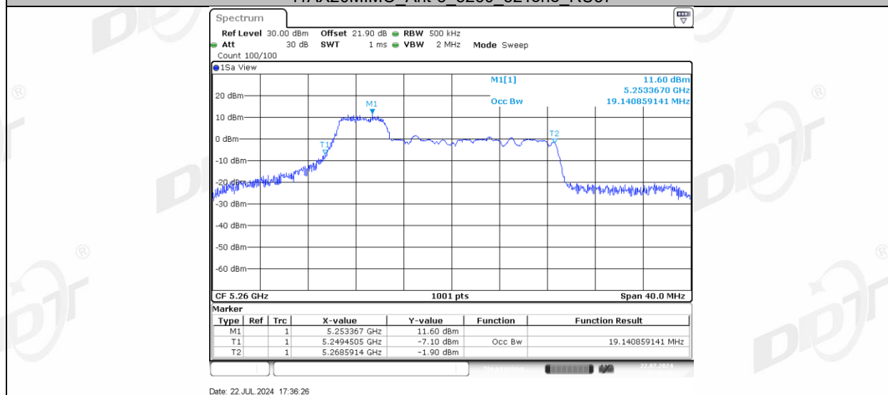
11AX20MIMO Ant-3 5260 52Tone RU39
