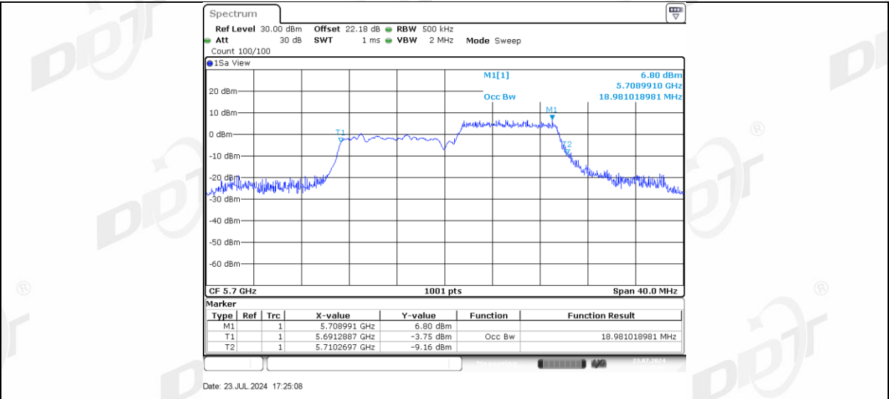
11AX20MIMO Ant-3 5700_26Tone_RU0
