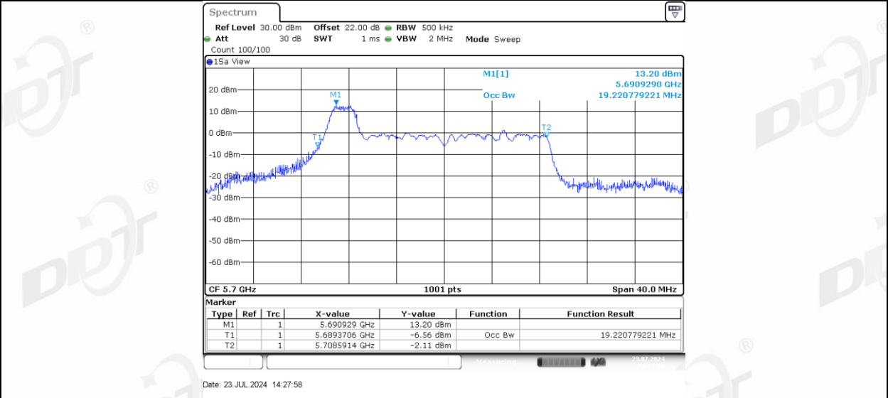
11AX20MIMO Ant-3 5700_26Tone_RU4
