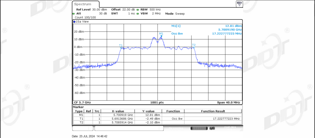
11AX20MIMO Ant-3 5700_26Tone_RU8
