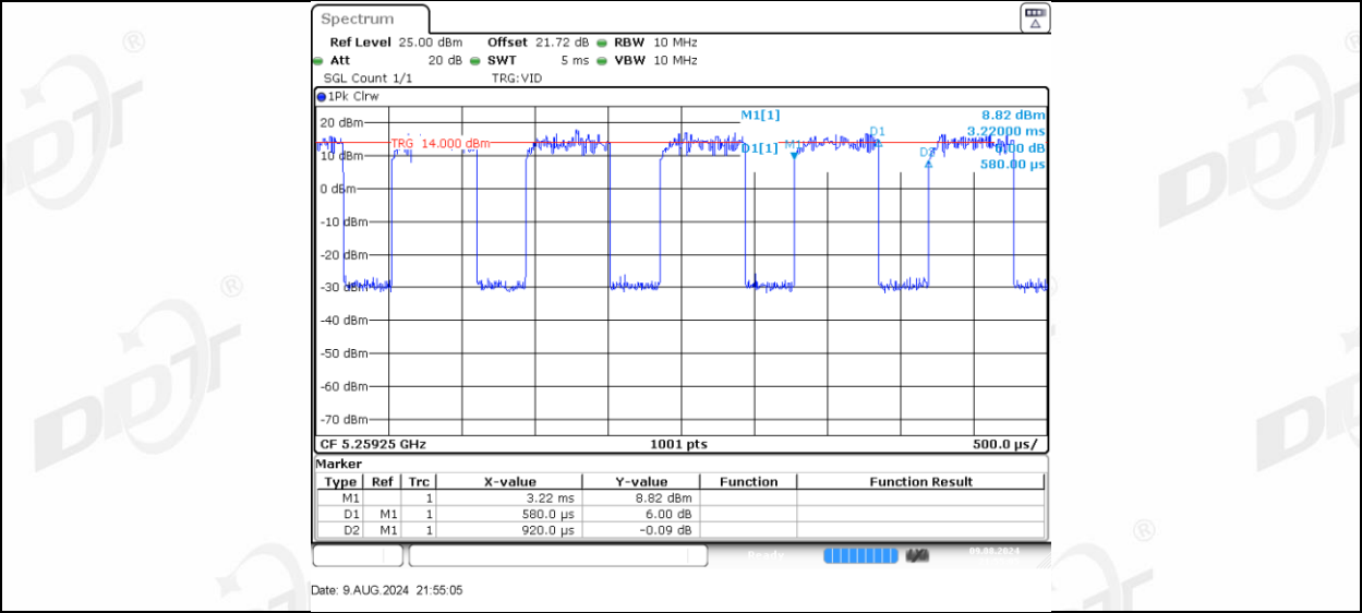
11AX20MIMO Ant-1_5260_26Tone_RU8
