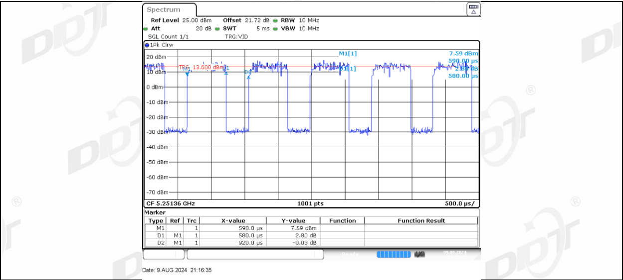
11AX20MIMO Ant-1_5260_26Tone_RU4
