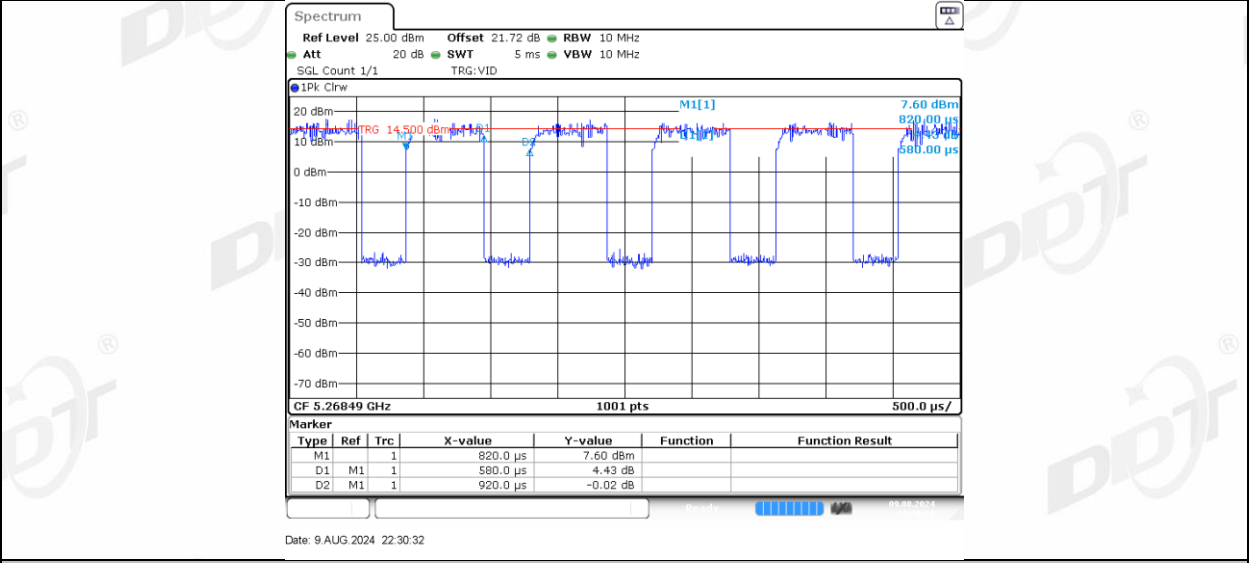
11AX20MIMO Ant-1_5260_52Tone_RU37
