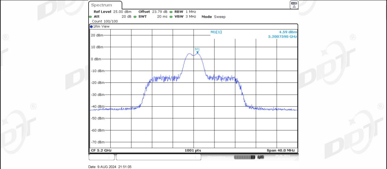
11AX20MIMO Ant-1_5200_26Tone_RU8
