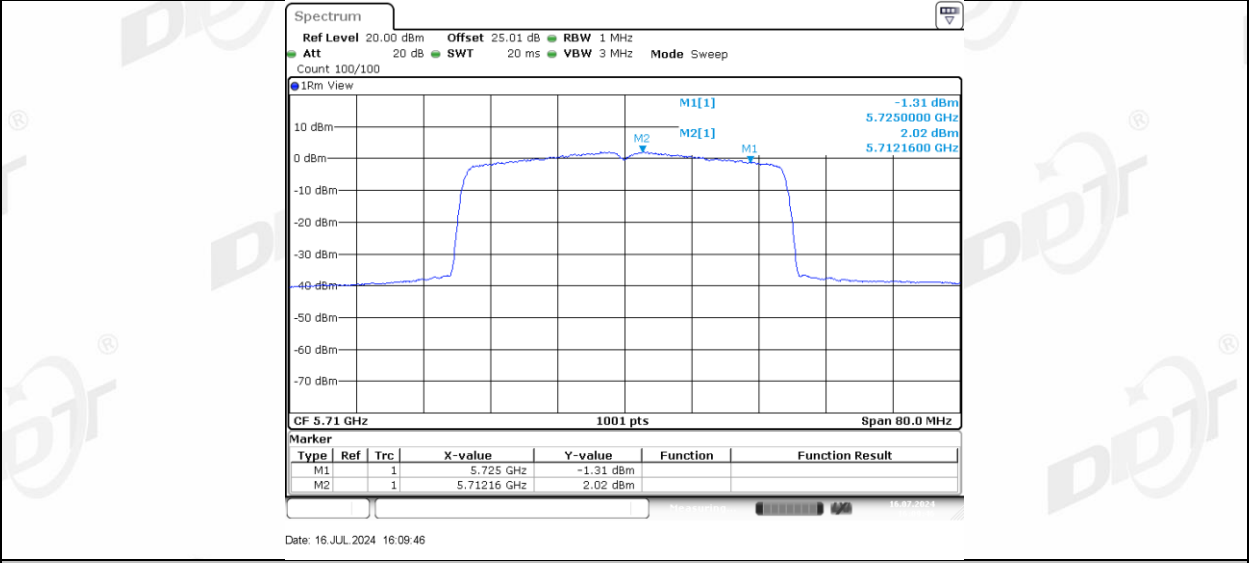
11AX40MIMO Ant-1_5710_UNII-3
