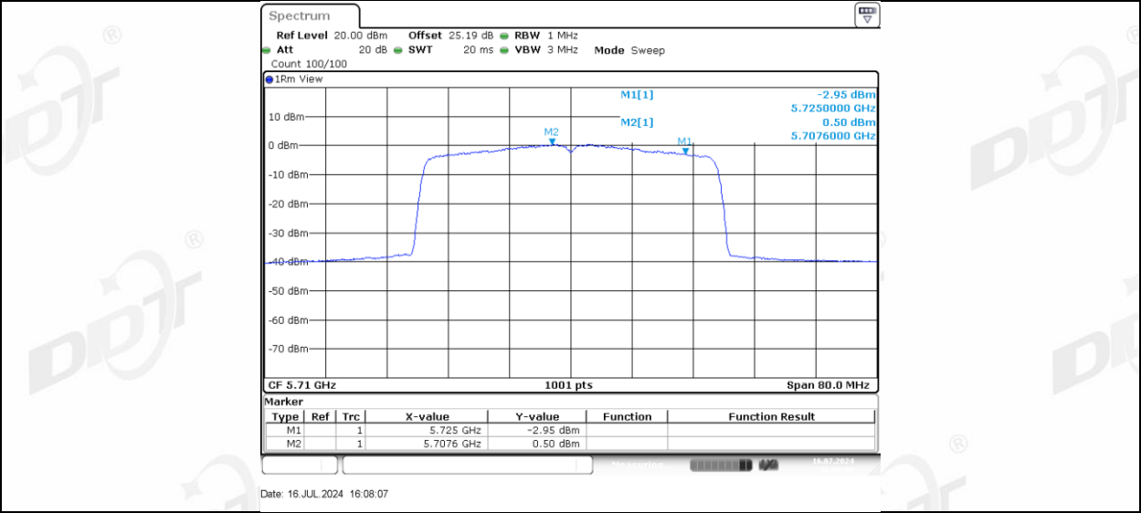
11AX40MIMO Ant-3_5710_UNII-2C
