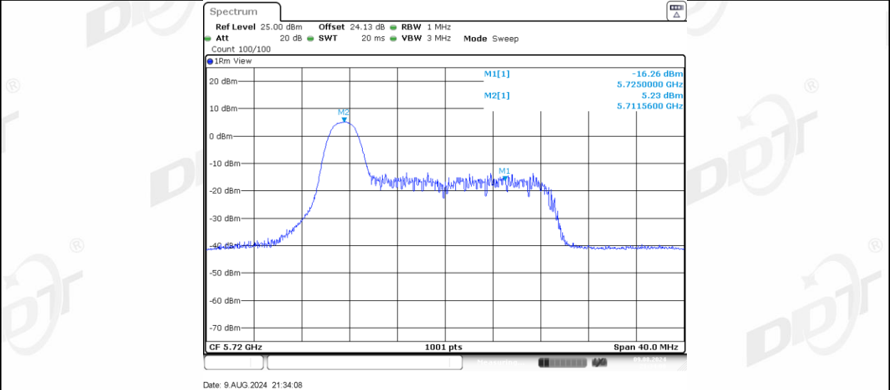
11AX20MIMO Ant-3_5720_UNII-2C_26Tone_RU4
