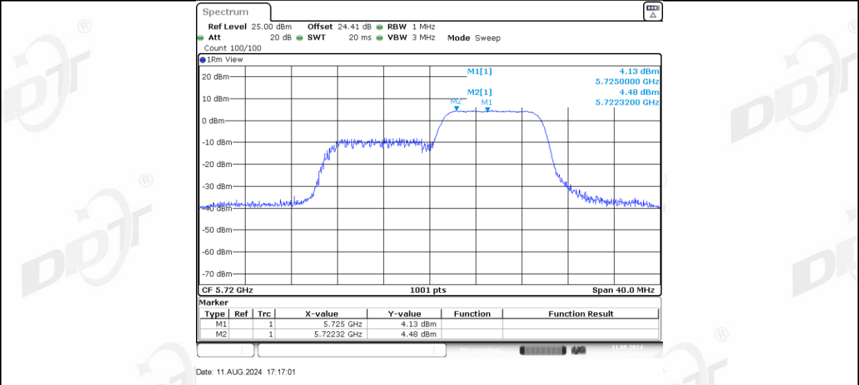
11AX20MIMO Ant-3_5720_UNII-2C_26Tone_RU0
