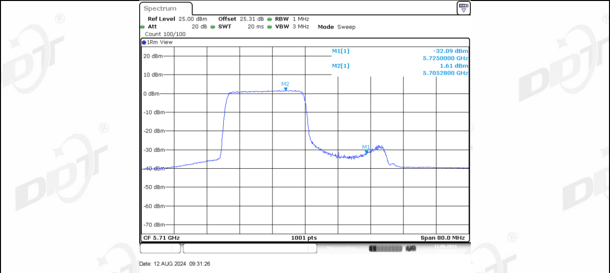
11AX40MIMO Ant-3 5710 UNII-2C 242Tone RU62
