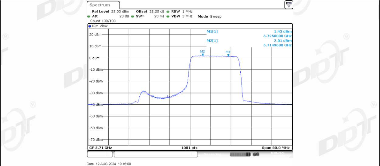
11AX40MIMO Ant-1 5710 UNII-3 106Tone RU53
