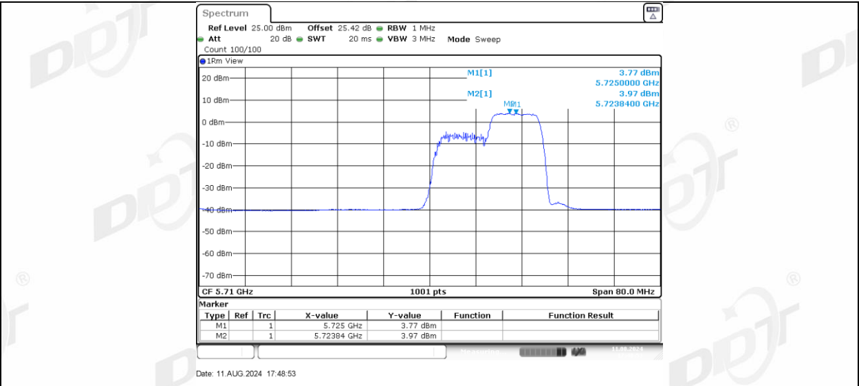
11AX40MIMO Ant-3 5710 UNII-2C 242Tone RU61
