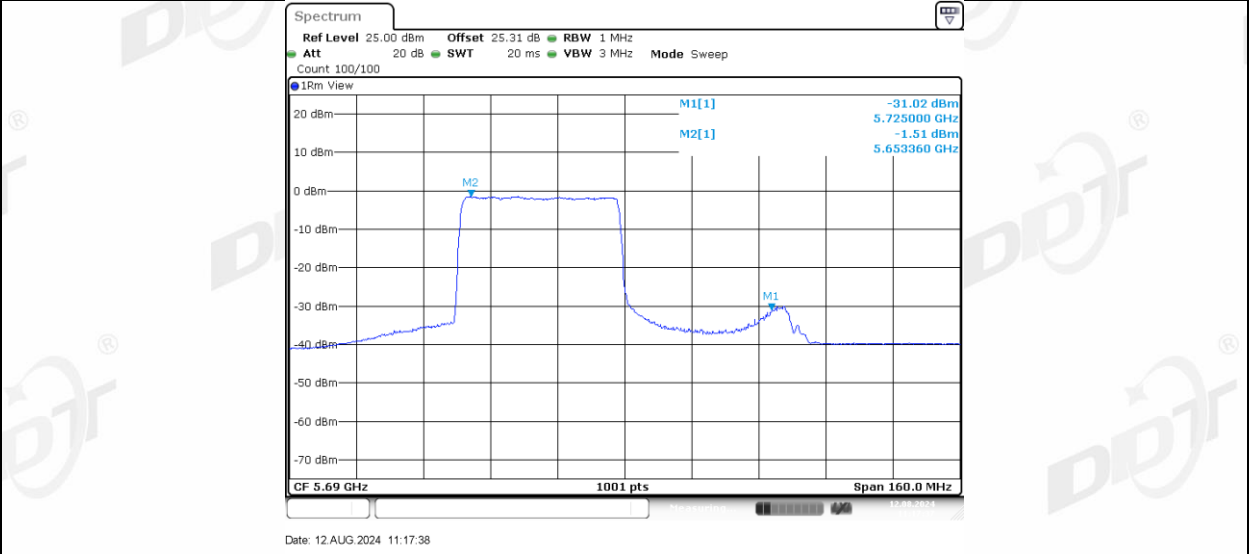
11AX80MIMO Ant-3 5690 UNII-2C 484Tone RU66
