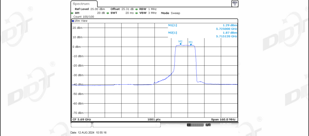
11AX80MIMO Ant-3 5690 UNII-2C 484Tone RU65
