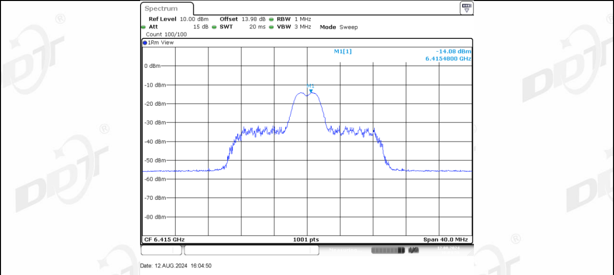
11AX20MIMO Ant-1_6415_26Tone_RU6
