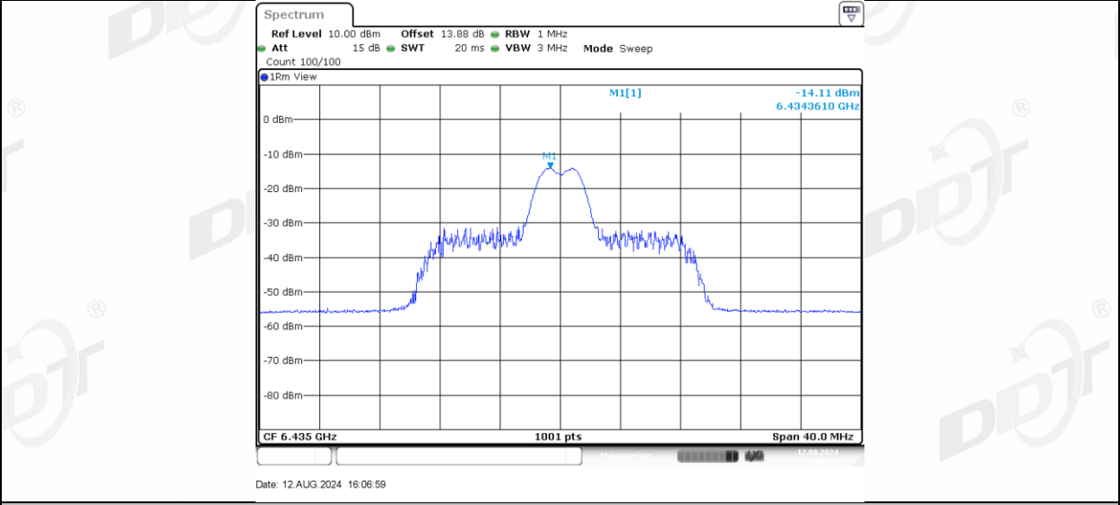
11AX20MIMO Ant-1_6435_26Tone_RU8
