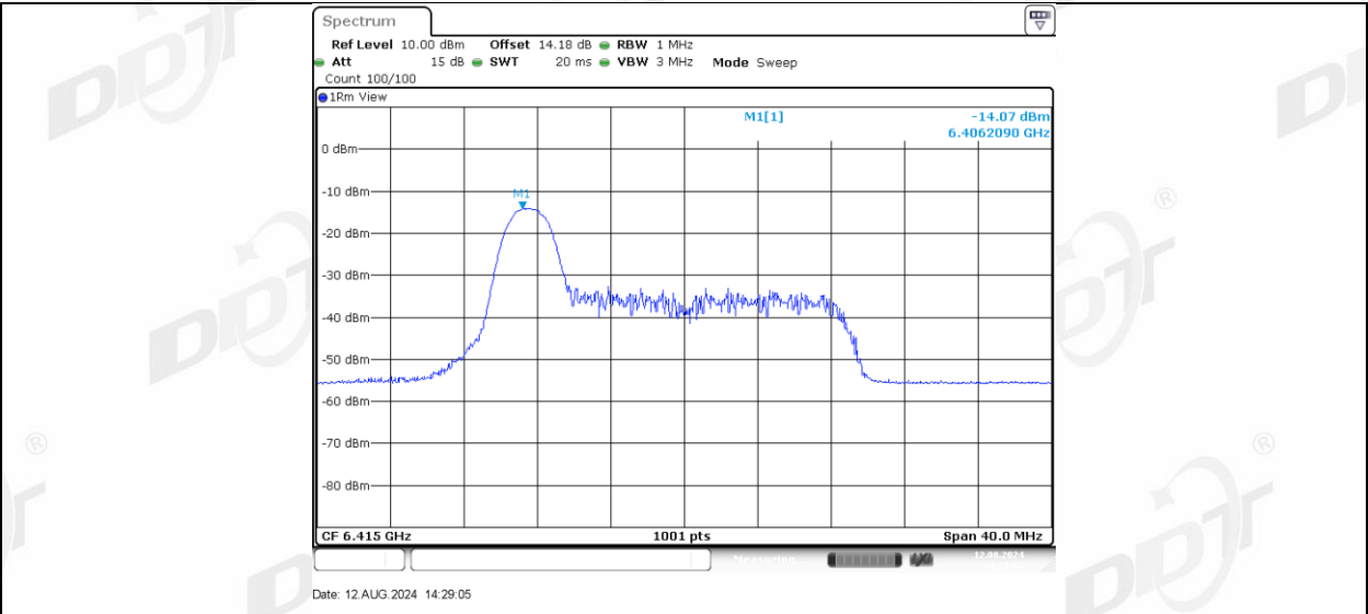
11AX20MIMO Ant-1_6415_26Tone_RU4
