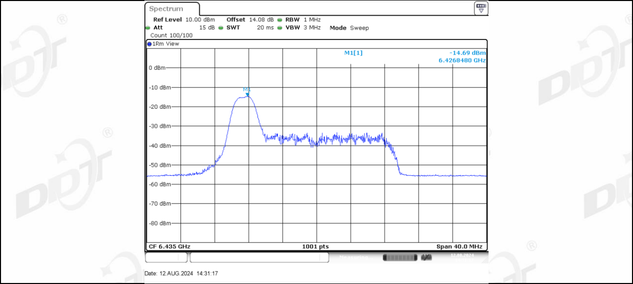
11AX20MIMO Ant-1_6435_26Tone_RU4
