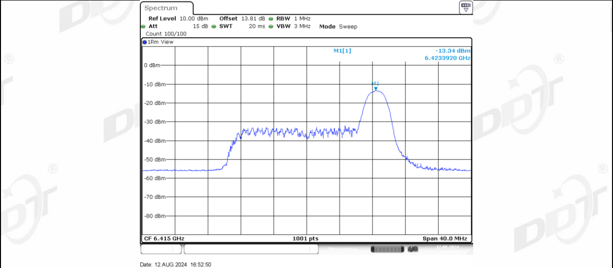
11AX20MIMO Ant-1_6415_52Tone_RU37
