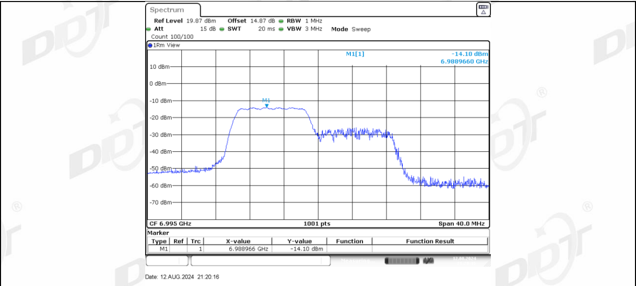
11AX20MIMO Ant-1_6995_106Tone_RU54
