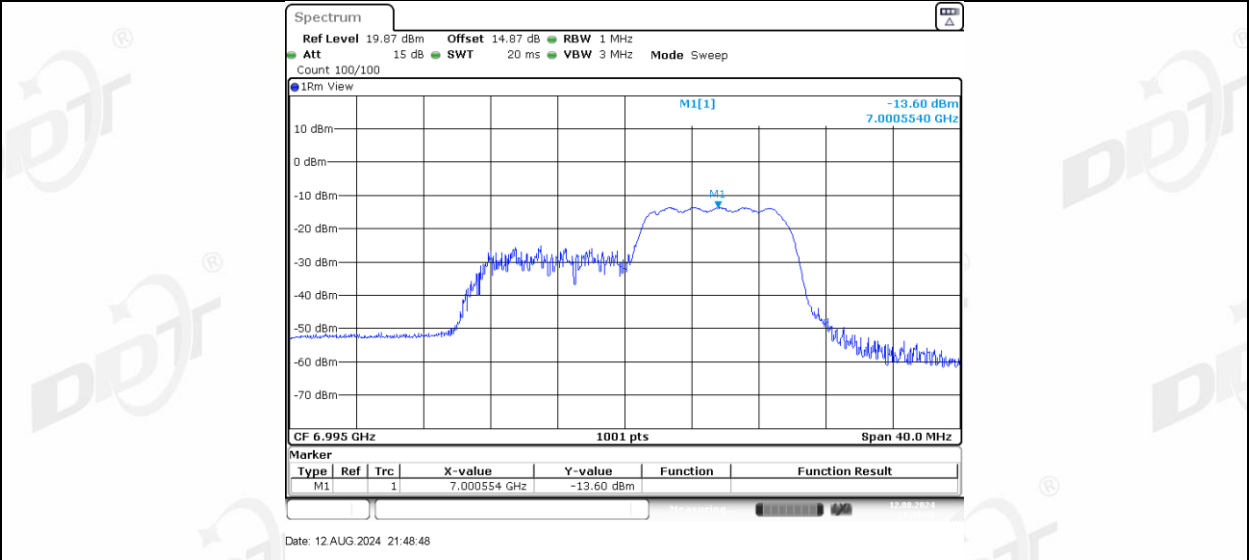
11AX20MIMO Ant-3_6995_26Tone_RU0
