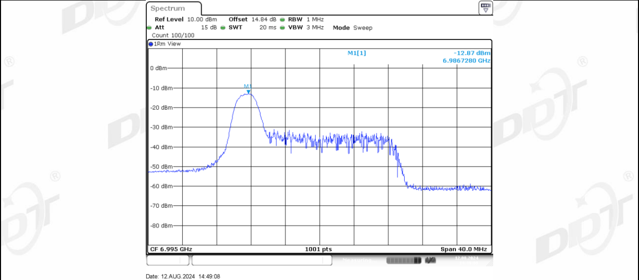
11AX20MIMO Ant-3_6995_26Tone_RU4
