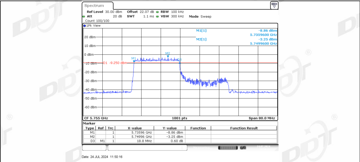
11AX40MIMO Ant-1_5755_242Tone_RU62
