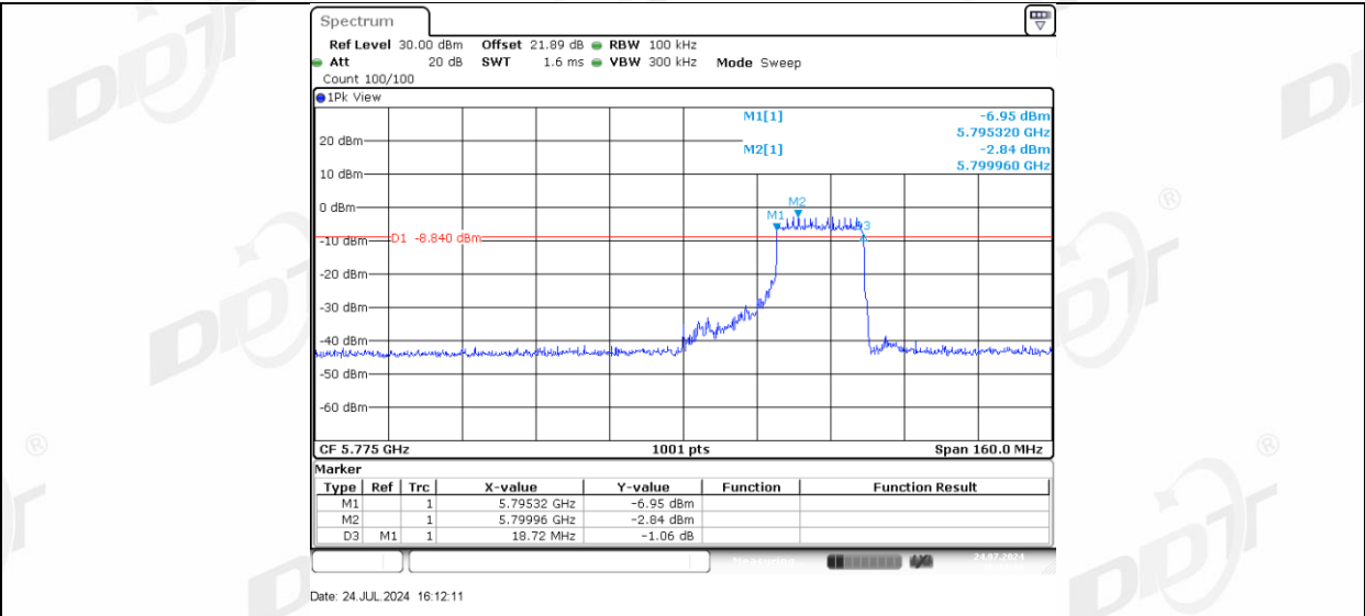
11AX80MIMO Ant-1_5775_484Tone_RU65
