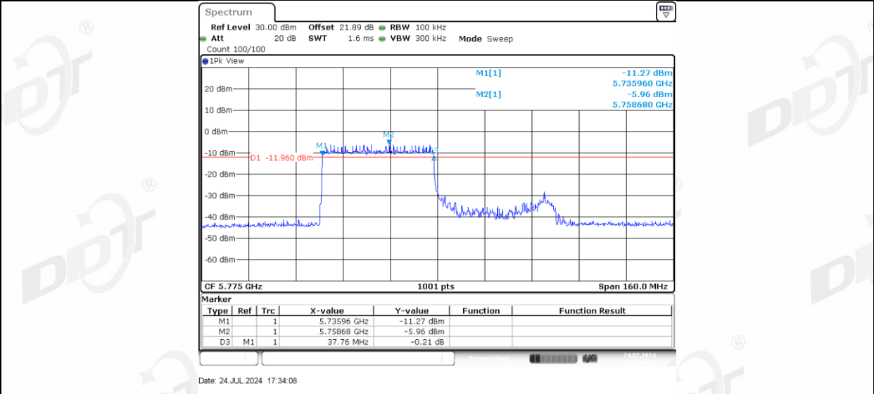
11AX80MIMO Ant-1_5775_484Tone_RU66
