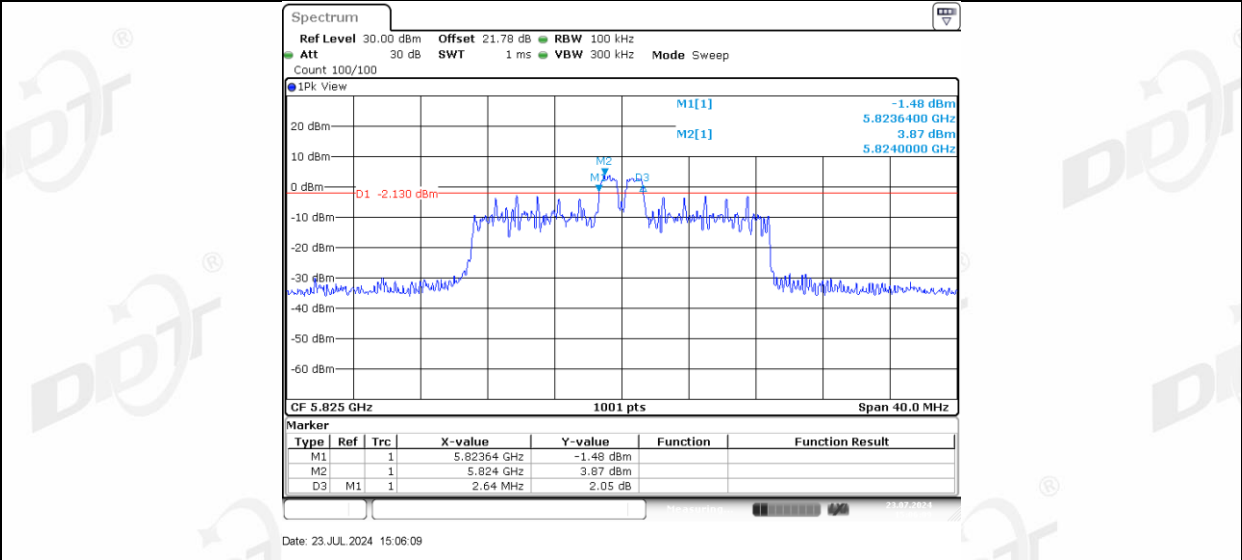
11AX20MIMO Ant-1_5825_26Tone_RU8
