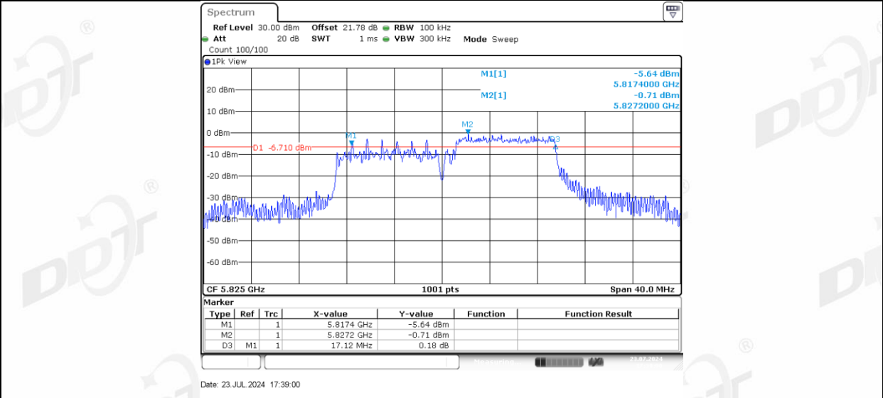
11AX20MIMO Ant-3_5825_26Tone_RU0
