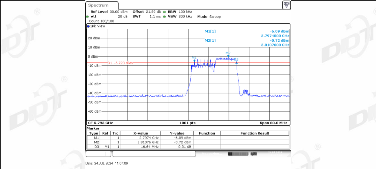
11AX40MIMO Ant-1_5795_242Tone_RU61
