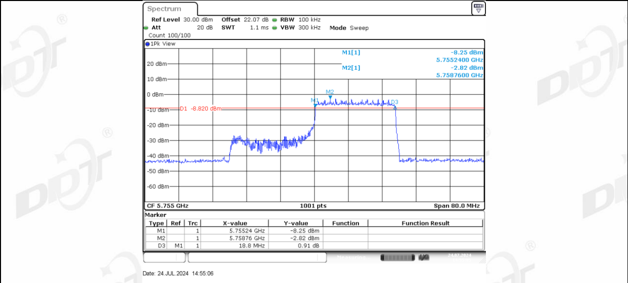
11AX40MIMO Ant-3_5755_106Tone_RU53
