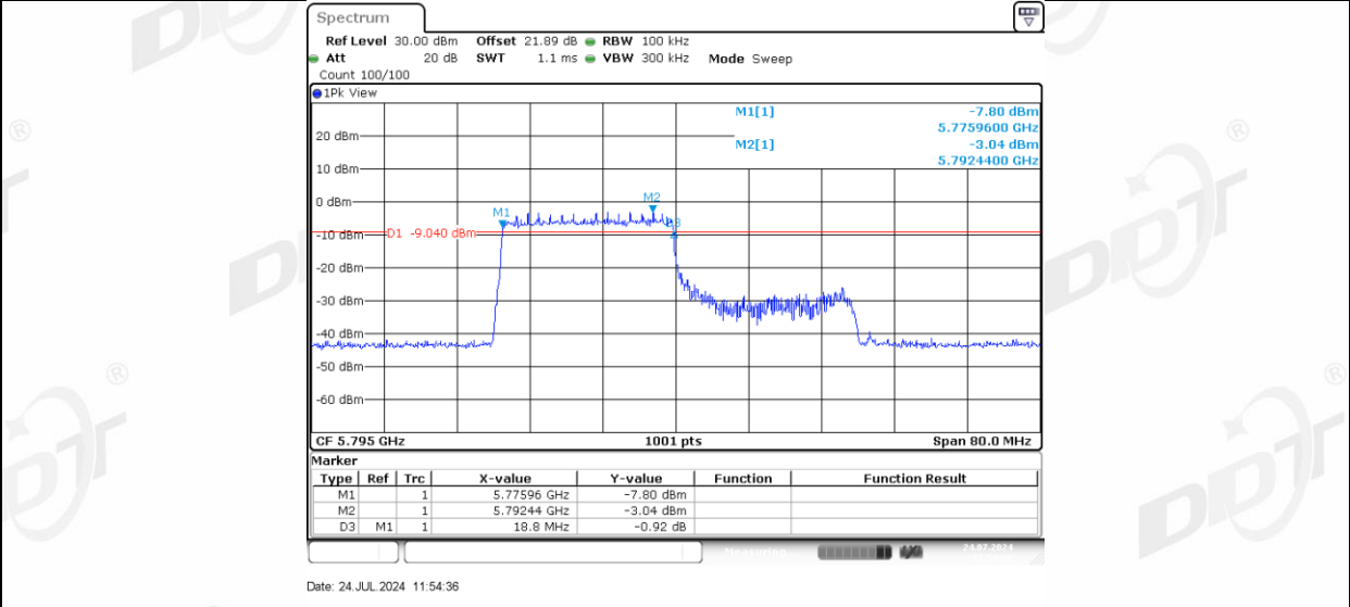
11AX40MIMO Ant-1_5795_242Tone_RU62
