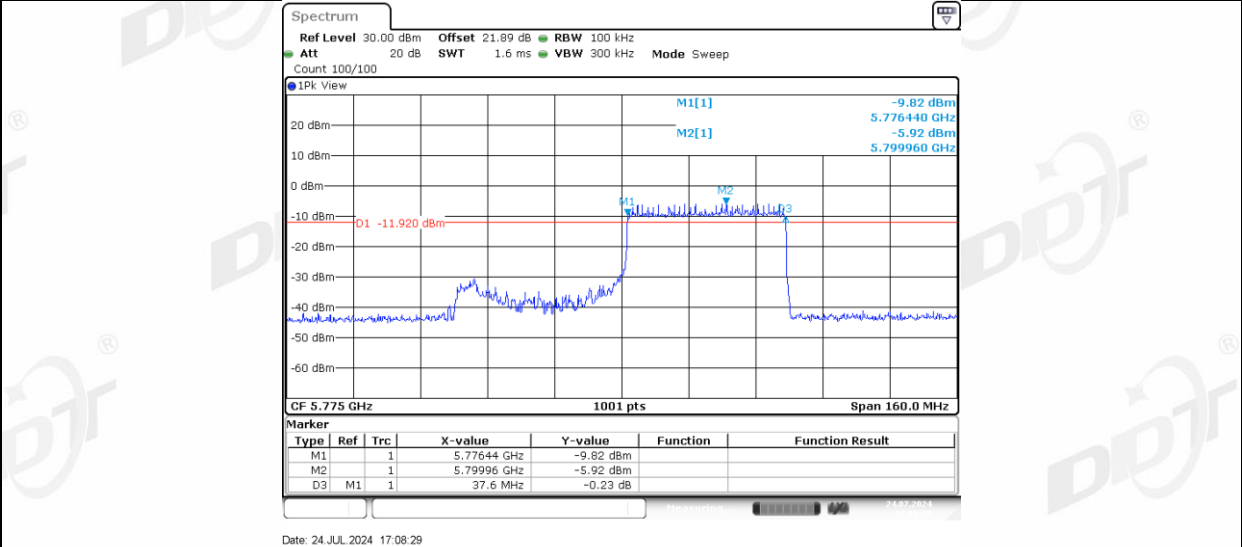
11AX80MIMO Ant-3_5775_242Tone_RU61
