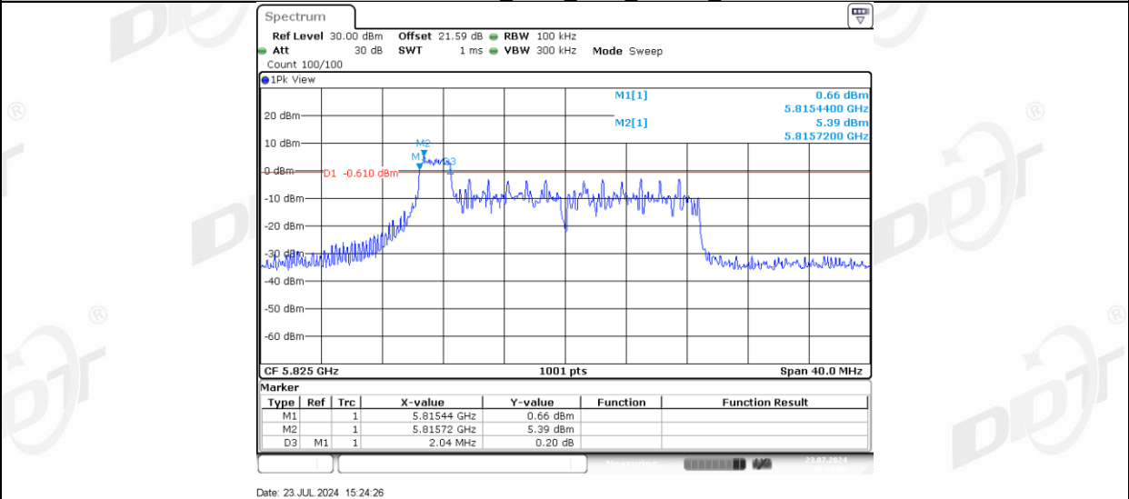
11AX20MIMO Ant-3_5825_26Tone_RU4
