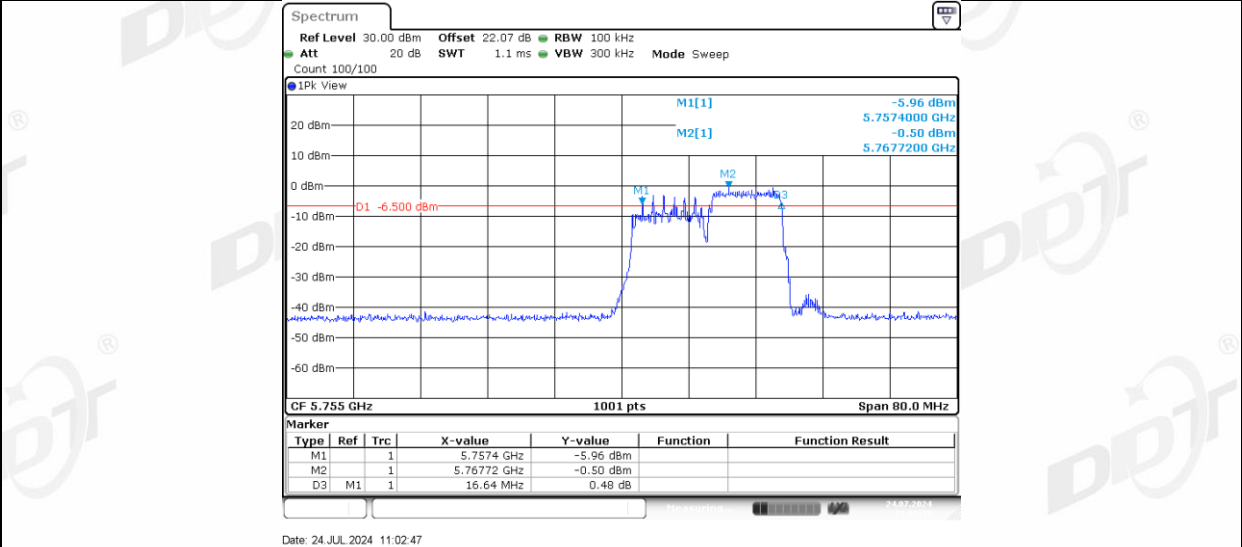
11AX40MIMO Ant-1_5755_242Tone_RU61
