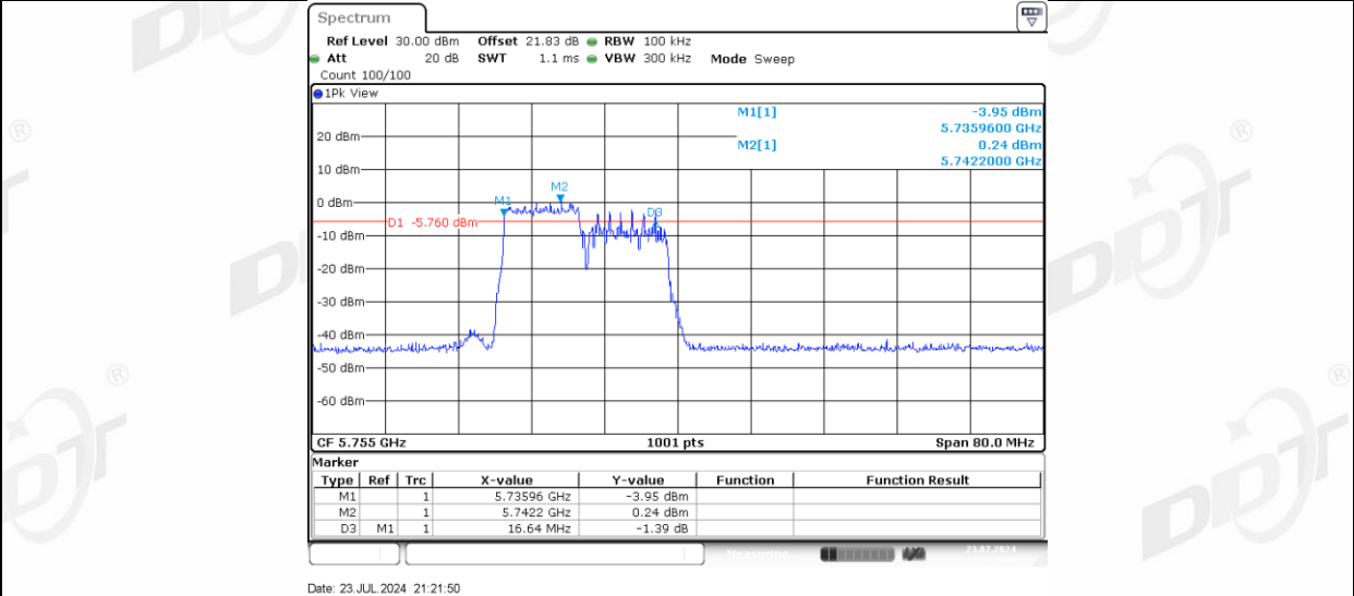
11AX40MIMO Ant-3_5755_106Tone_RU56
