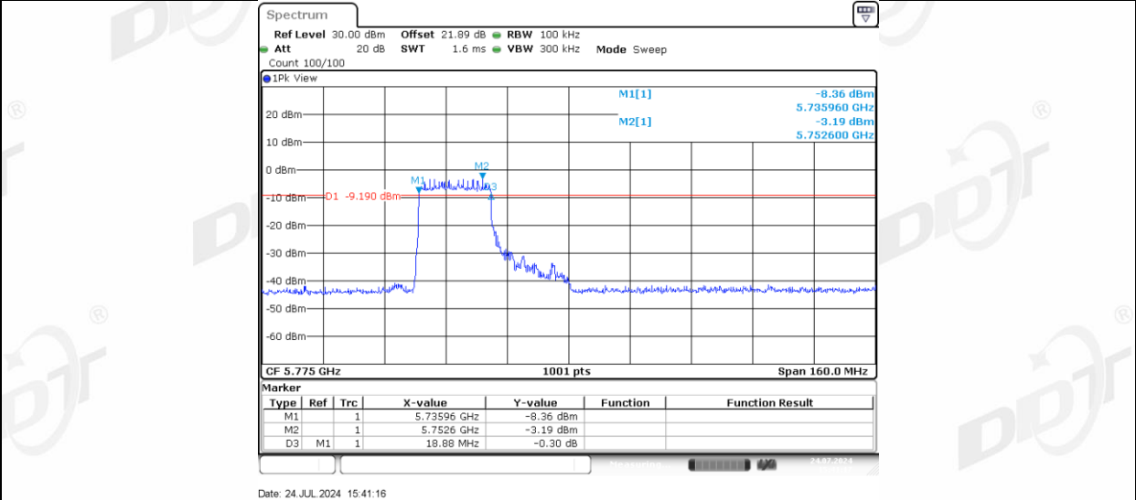
11AX80MIMO Ant-1_5775_242Tone_RU64
