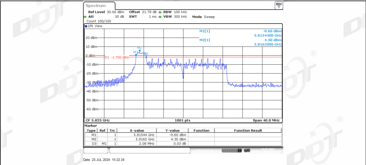
11AX20MIMO Ant-1_5825_26Tone_RU4
