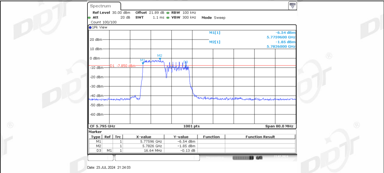
11AX40MIMO Ant-1_5795_106Tone_RU56
