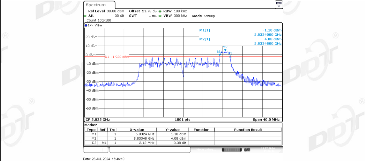
11AX20MIMO Ant-1_5825_52Tone_RU37
