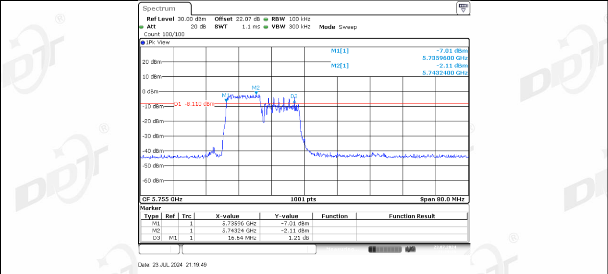
11AX40MIMO Ant-1_5755_106Tone_RU56
