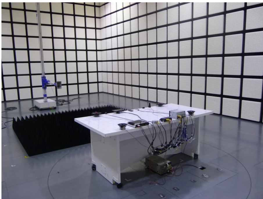
Rear view (1-15 GHz)
