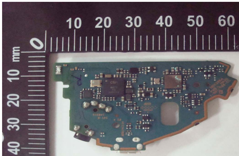
Main PWB (Back)
