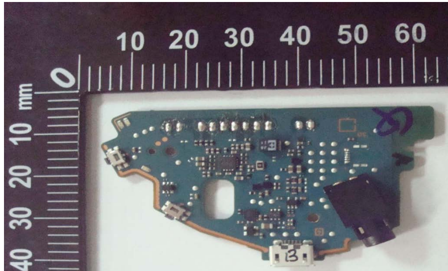
Main PWB (Front)
