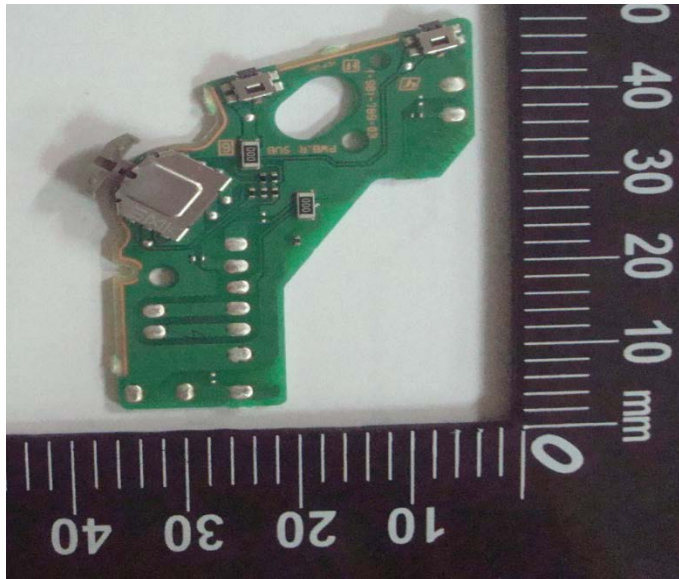
R Sub PWB (Front)
