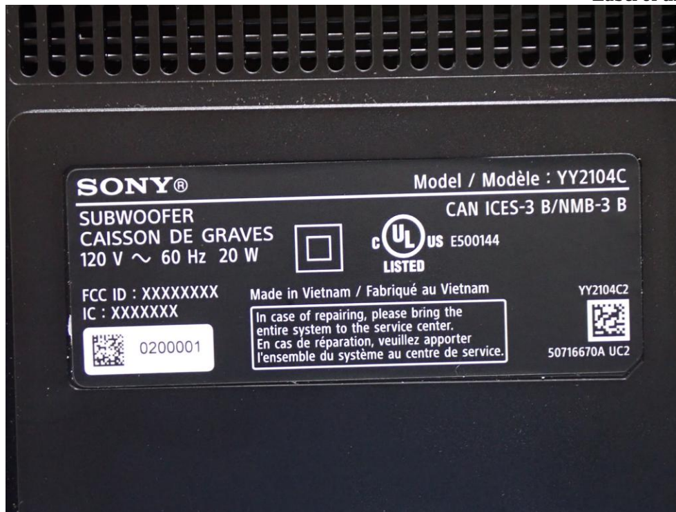
Figure 11 Label of the EUT(YY2104C2)
