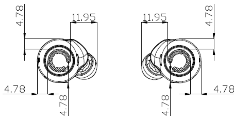
Figure F-1 Antenna Location
